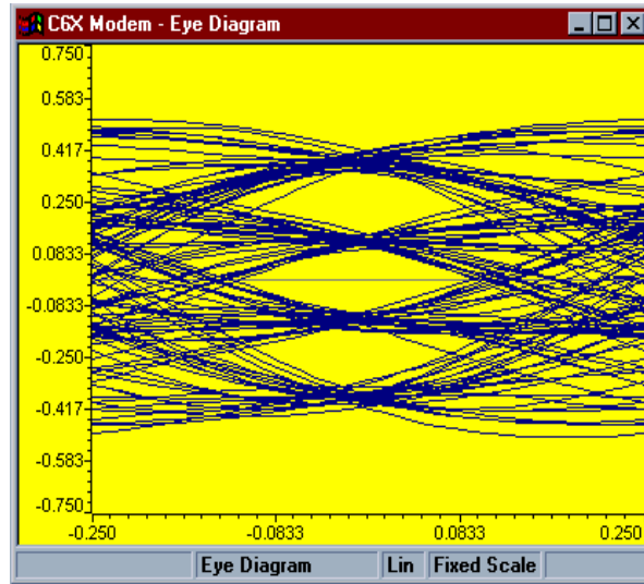
Figure 12. Eye Diagram
