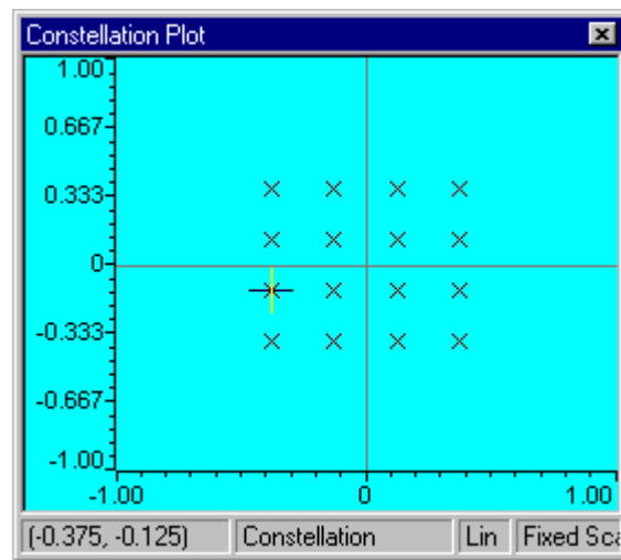
Figure 11. Constellation Plot
