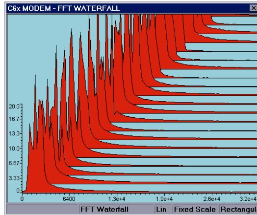
Figure 10. FFT Waterfall
