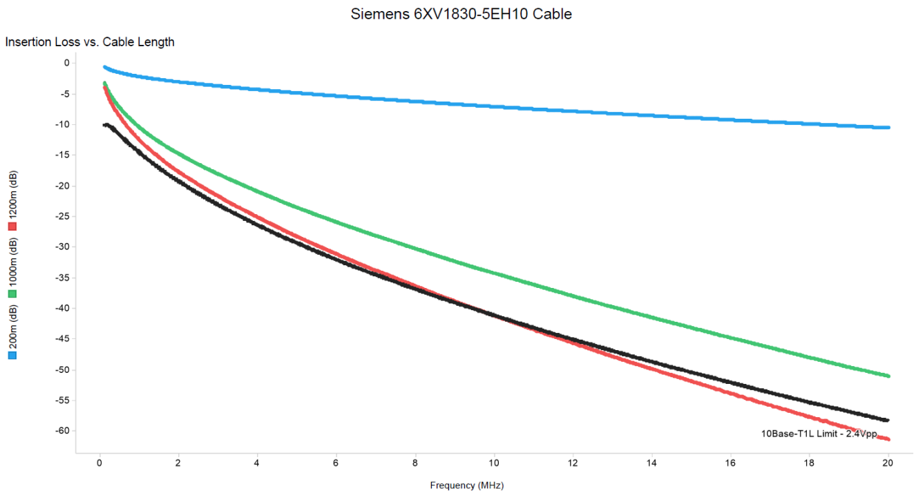
Figure 4-3. Siemens 6XV1830-5EH10 Cable
