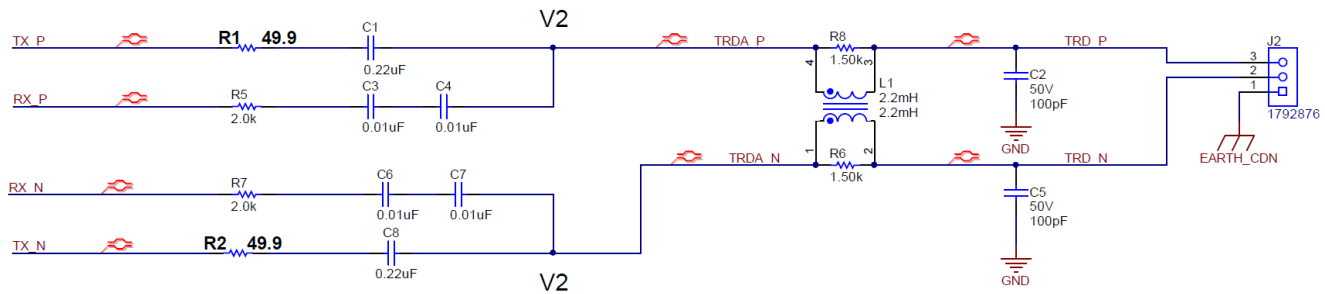
Figure 4-1. 100 ohm Characteristic Impedance Cable Design
