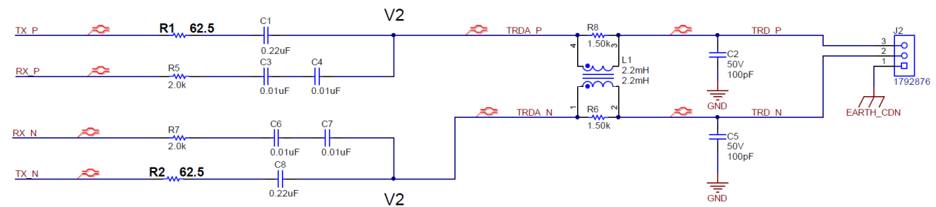
Figure 4-2. 125 ohm Characteristic Impedance Cable Design
