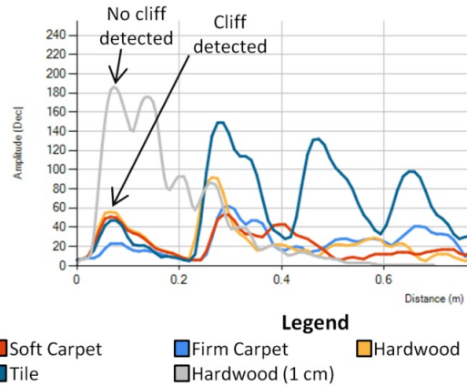
Figure 5. Cliff Detection at 20 cm
