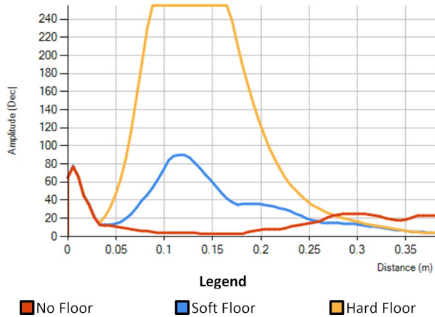
Figure 3. Floor-Type Detection
