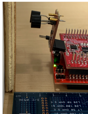
Figure 2. BOOSTXL-PGA460 Test Setup
