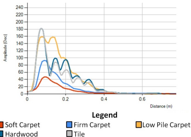
Figure 4. Echo Response Across Different Surfaces
