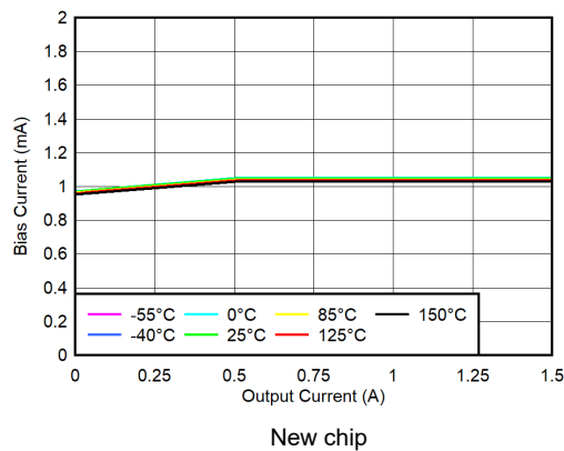
Figure 5-23. BIAS Pin Current vs Output Current and Temperature ( T_J )
