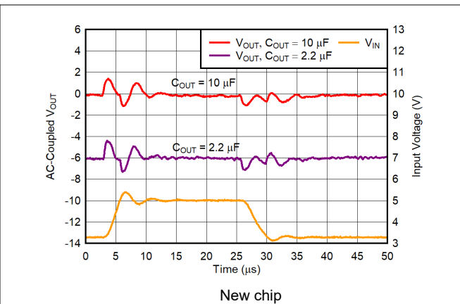
Figure 5-33. V BIAS Line Transient
