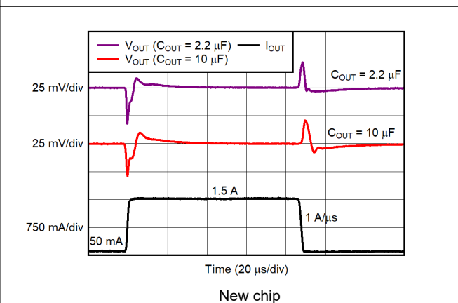
Figure 5-37. Output Load Transient Response
