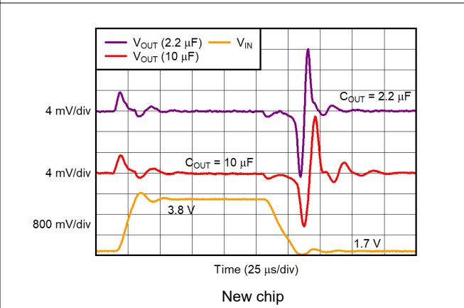
Figure 5-35. V IN Line Transient
