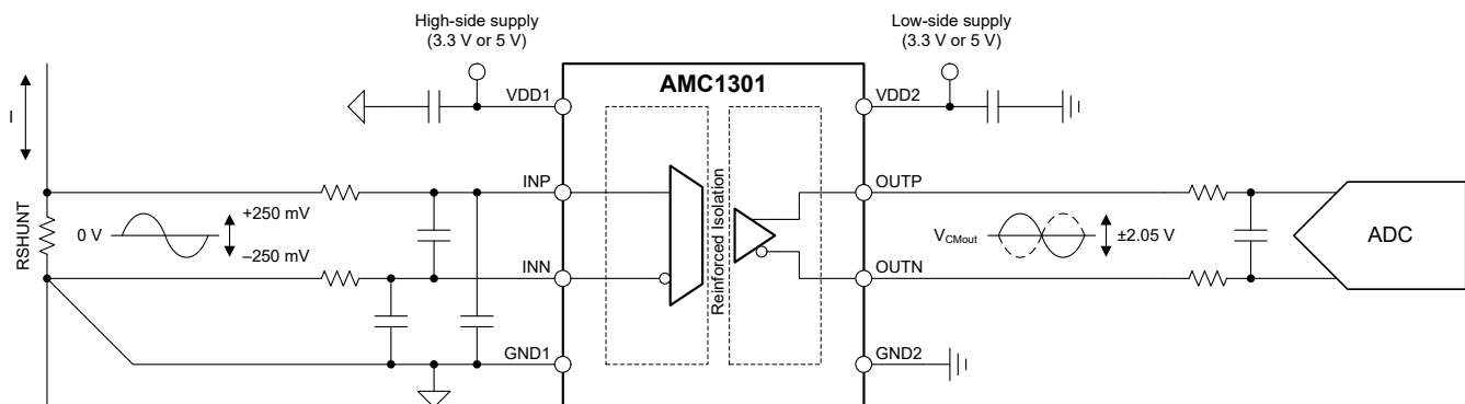
Simplified Schematic
