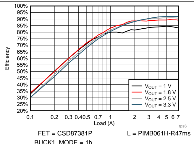
Figure 4-4. Example BUCK1 Efficiency at V_{IN} = 13\text{ V} in Forced PWM Mode
