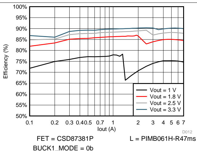
Figure 4-5. Example BUCK1 Efficiency at V_{IN} = 18\text{ V} In Auto Mode
