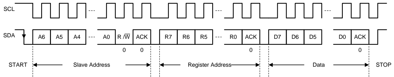
Figure 5-18. I²C Interface WRITE to TPS650861 in F/S Mode
