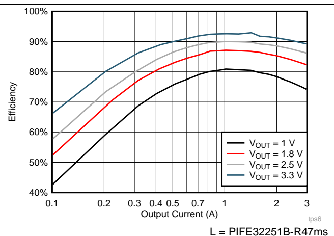
Figure 4-6. Example BUCK3 Efficiency at V_{IN} = 5\text{ V}
