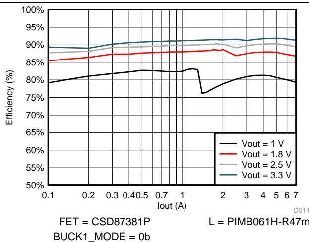
Figure 4-3. Example BUCK1 Efficiency at V_{IN} = 13\text{ V} In Auto Mode
