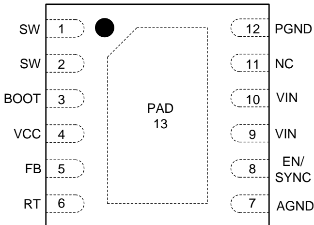
Pin Functions
