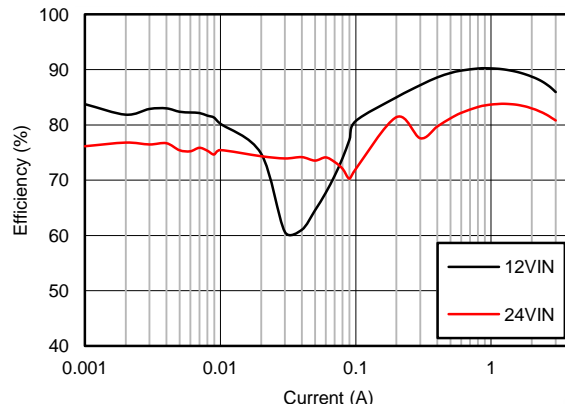
Figure 80. Efficiency
