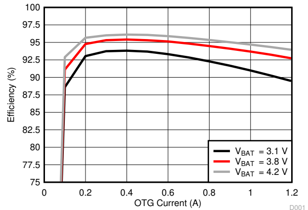
图 7-2. Efficiency vs. OTG Current
