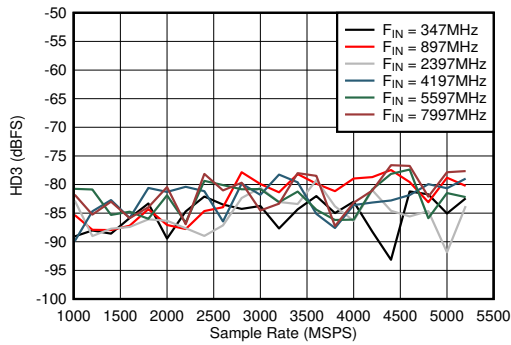
图 6-55. Dual Channel Mode: HD3 vs Sample Rate and Input Frequency
