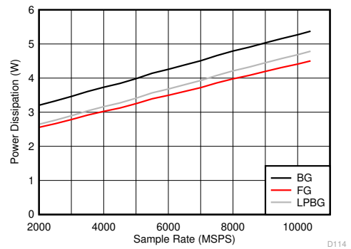
图 6-128. DES Mode: Power Dissipation vs Sample Rate
