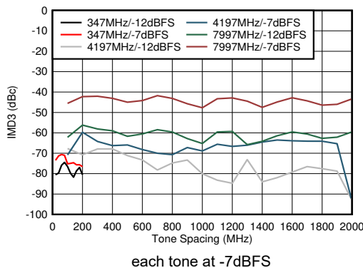
图 6-101. DES Mode: IMD3 vs Tone Spacing
