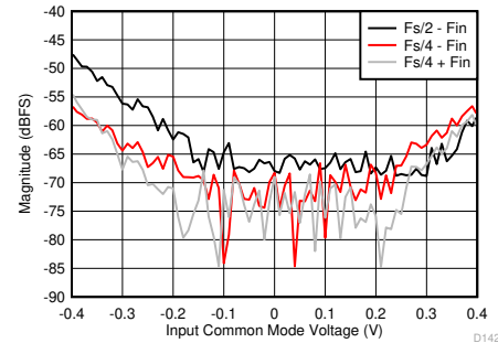
图 6-98. F_s/2 - F_{\text{IN}} and F_s/4 \pm F_{\text{IN}} vs Input Common Mode Voltage
