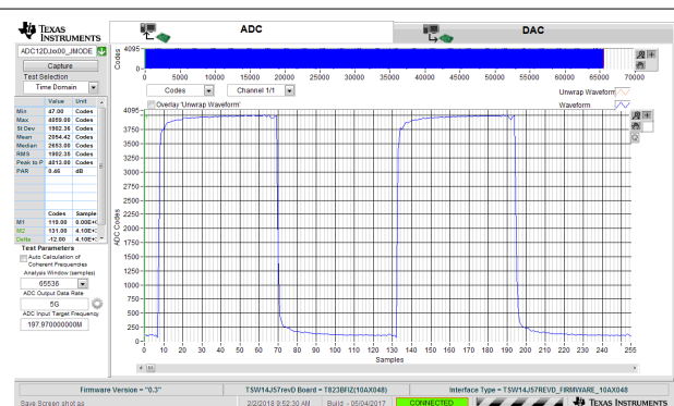
图 8-7. 40-MHz, Square-Wave Time Domain for 5-GSPS, Single-Channel Oscilloscope
