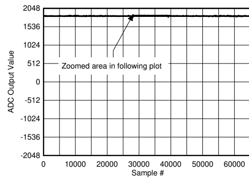
图 6-144. Background Calibration Core Transition (DC Signal)
