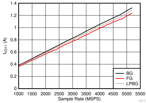
图 6-133. Dual Channel Mode: I_{VD11} vs Sample Rate
