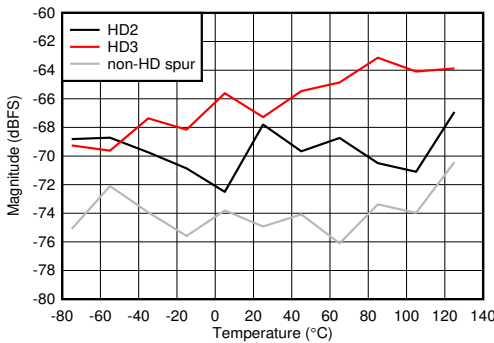
图 6-87. DES Mode: HD2, HD3 and Worst non-HD Spur vs Temperature
