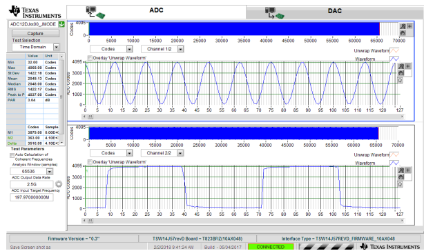
图 8-11. 200-MHz, Sine-Wave (Channel A) and 40-MHz, Square-Wave (Channel B) Time Domain for 5-GSPS, Single-Channel Oscilloscope
