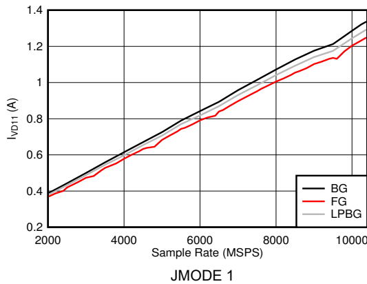
图 6-123. DES Mode: I_{VD11} vs Sample Rate
