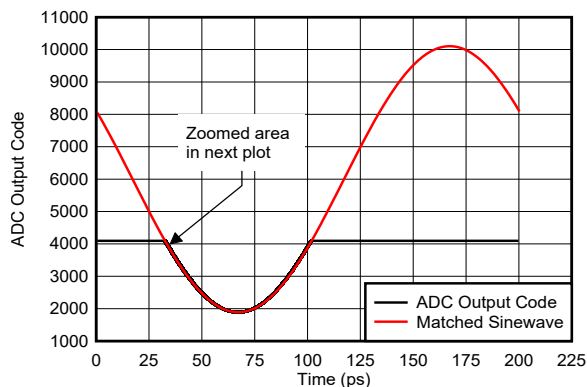
图 6-148. Sinewave Overdrive Recovery
