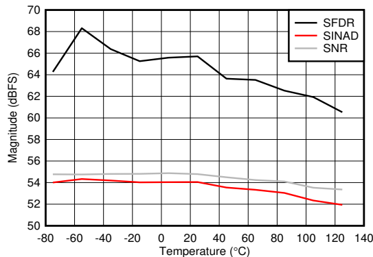
图 6-89. Dual Channel Mode: SNR, SINAD and SFDR vs Temperature
