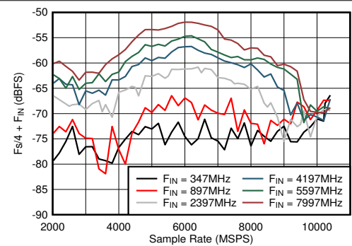
图 6-42. DES Mode: \text{Fs}/4 + F_{\text{IN}} vs Sample Rate and Input Frequency
