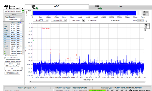
图 8-9. 200-MHz, Sine-Wave Frequency Domain (FFT) for 5-GSPS, Single-Channel Oscilloscope
