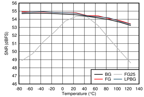
图 6-86. DES Mode: SNR vs Temperature and Calibration Mode
