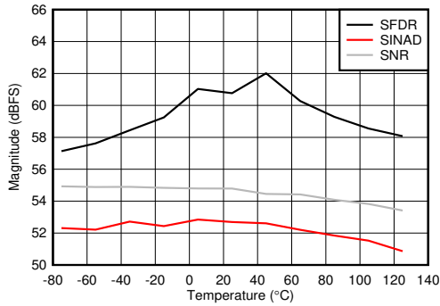
图 6-85. DES Mode: SNR, SINAD and SFDR vs Temperature
