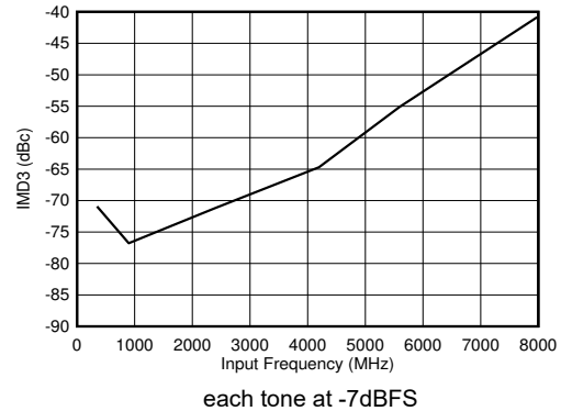
图 6-104. Dual Channel Mode: IMD3 vs Input Frequency
