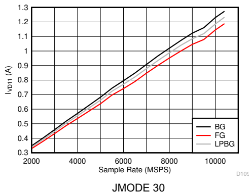
图 6-125. DES Mode: I_{VD11} vs Sample Rate
