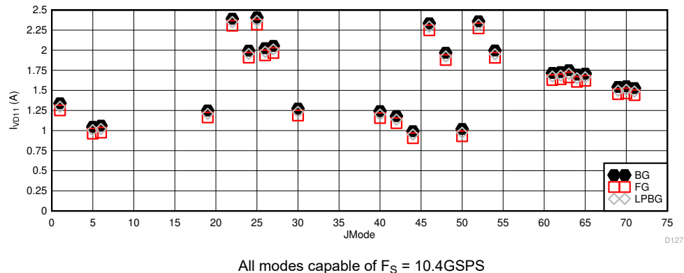
图 6-111. DES Mode: I_{VD11} vs JMODE at 10.4GSPS
