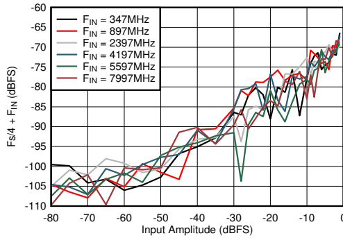
图 6-67. DES Mode: F_s/4 + F_{\text{IN}} vs Input Amplitude and Frequency
