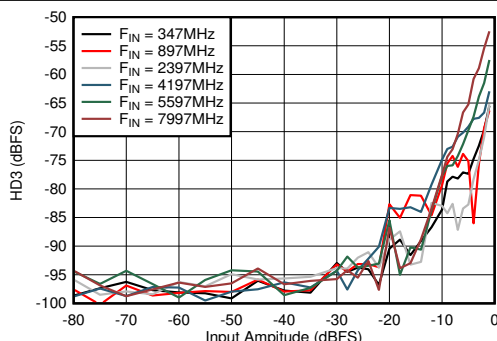
图 6-63. DES Mode: HD3 vs Input Amplitude and Frequency
