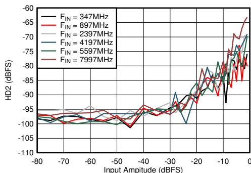
图 6-61. DES Mode: HD2 vs Input Amplitude and Frequency
