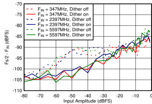
图 6-80. Dual Channel Mode: F_{\text{s}}/2 - F_{\text{IN}} vs Input Amplitude and Dither
