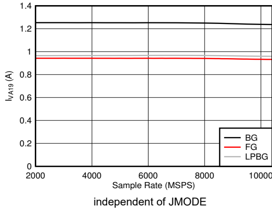
图 6-121. DES Mode: I_{VA19} vs Sample Rate
