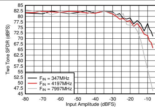
图 6-108. Dual Channel Mode: Two Tone SFDR vs Input Amplitude
