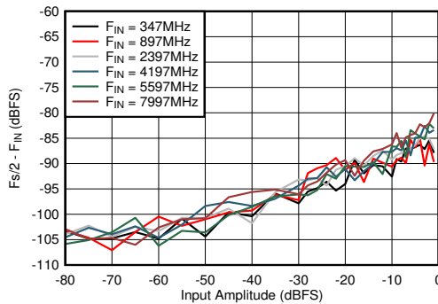
图 6-79. Dual Channel Mode: F_{\text{s}}/2 - F_{\text{IN}} vs Input Amplitude and Frequency
