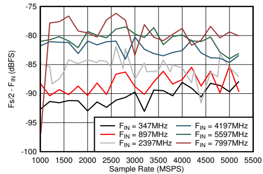
图 6-56. Dual Channel Mode: F_{\text{s}}/2 - F_{\text{IN}} vs Sample Rate and Input Frequency
