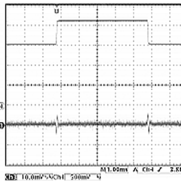
Figure 4. Load Transient
