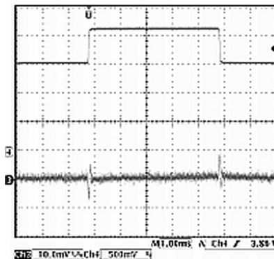
Figure 3. Load Transient
