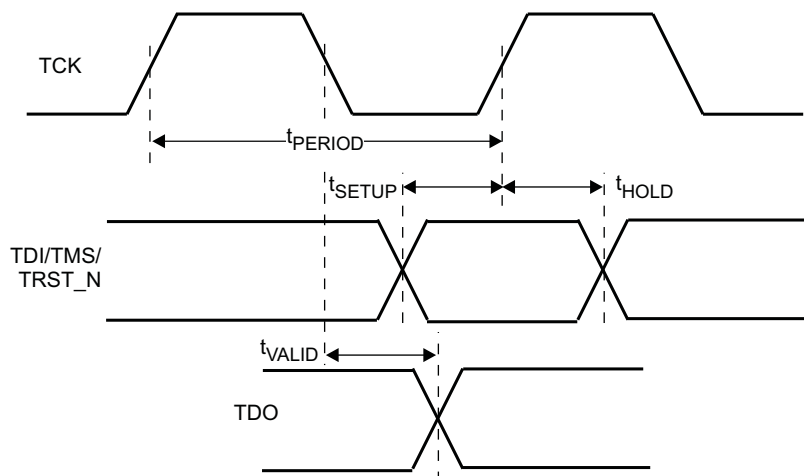
Figure 31. JTAG Timing
