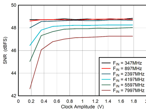
图 6-83. Dual Channel Mode: SNR vs Clock Amplitude
