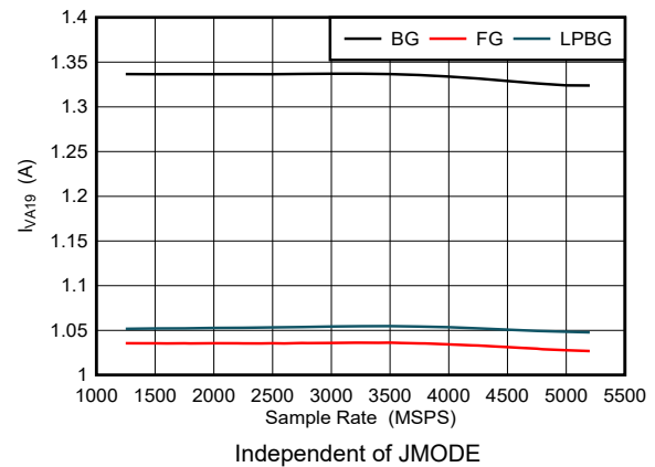
图 6-114. Dual Channel Mode: I_{VA19} vs Sample Rate
