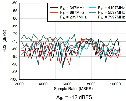
图 6-37. DES Mode: HD2 vs Sample Rate
