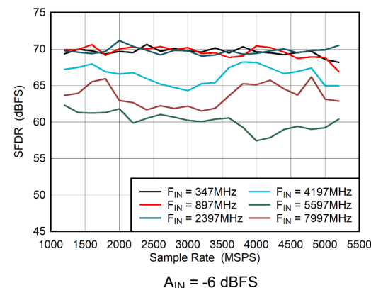
图 6-48. Dual Channel Mode: SFDR vs Sample Rate
