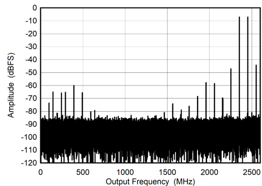
图 6-28. Dual Channel Mode: Two Tone FFT at 7997 MHz
