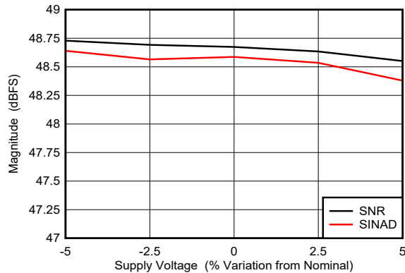
图 6-95. Dual Channel Mode: SNR and SINAD vs Supply Voltage
