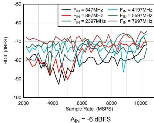
图 6-39. DES Mode: HD3 vs Sample Rate
