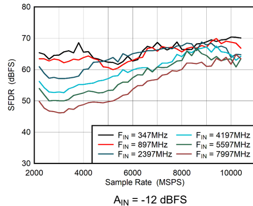
图 6-34. DES Mode: SFDR vs Sample Rate
