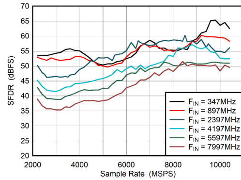
图 6-32. DES Mode: SFDR vs Sample Rate
