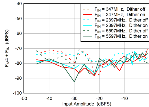
图 6-68. DES Mode: F_S/4 + F_{\text{IN}} vs Input Amplitude and Dither
