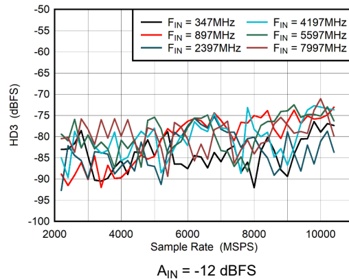
图 6-40. DES Mode: HD3 vs Sample Rate
