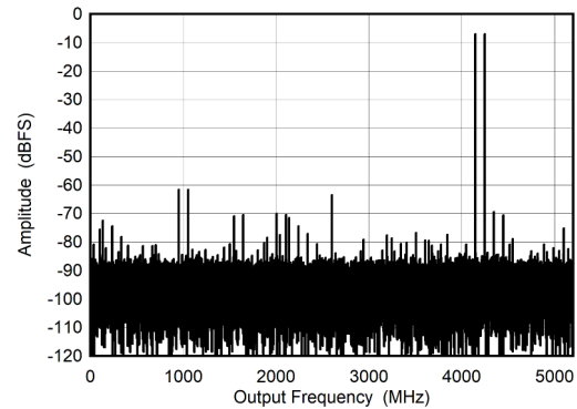
图 6-14. DES Mode: Two Tone FFT at 4197 MHz
