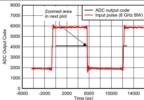
图 6-123. Pulse Overdrive Recovery
