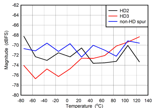
图 6-90. Dual Channel Mode: HD2, HD3 and Worst Spur vs Temperature
