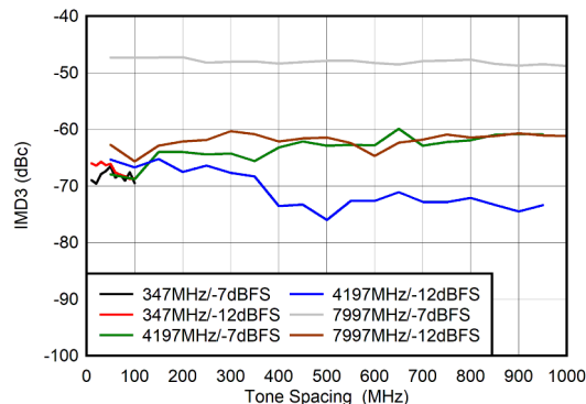
图 6-102. DES Mode: IMD3 vs Tone Spacing
