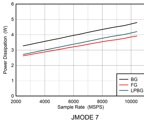
图 6-113. DES Mode: Power Dissipation vs Sample Rate
