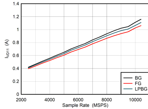
图 6-112. DES Mode: I_{VD11} vs Sample Rate
