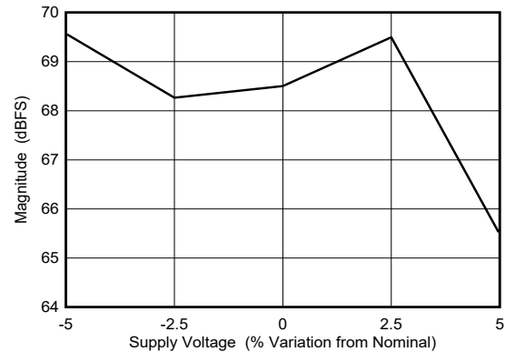
图 6-96. Dual Channel Mode: SFDR vs Supply Voltage
