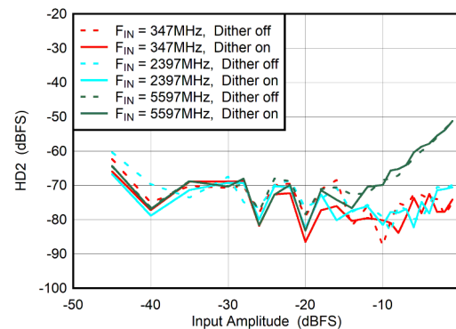
图 6-76. Dual Channel Mode: HD2 vs Input Amplitude and Dither
