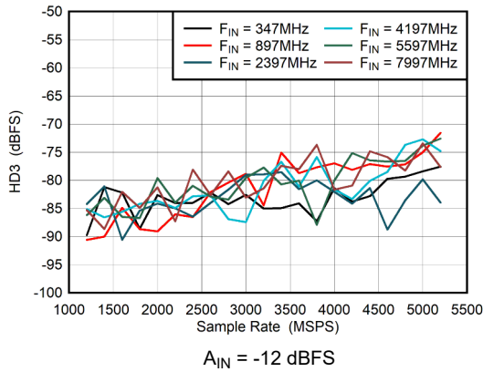
图 6-55. Dual Channel Mode: HD3 vs Sample Rate
