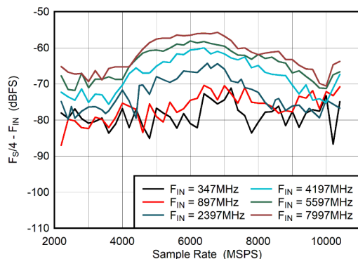
图 6-43. DES Mode: F_S/4 - F_{\text{IN}} vs Sample Rate
