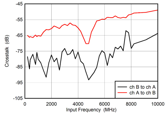
图 6-2. Crosstalk vs Input Frequency
