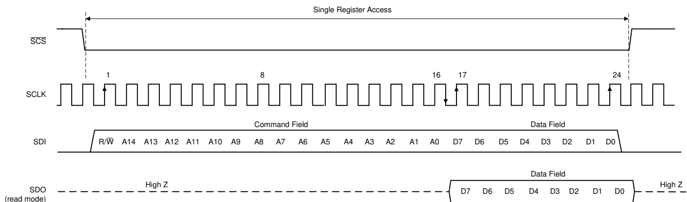
图 7-15. Serial Interface Protocol: Single Read/Write
