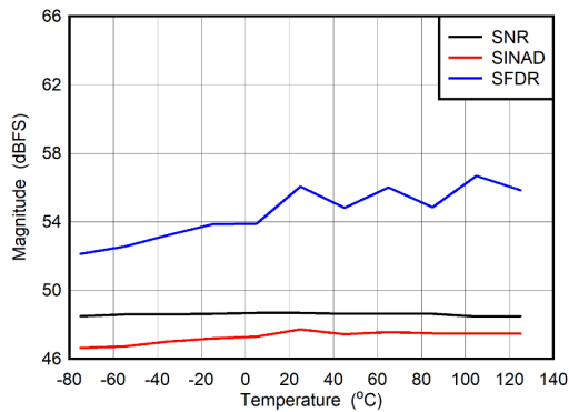
图 6-85. DES Mode: SNR, SINAD and SFDR vs Temperature
