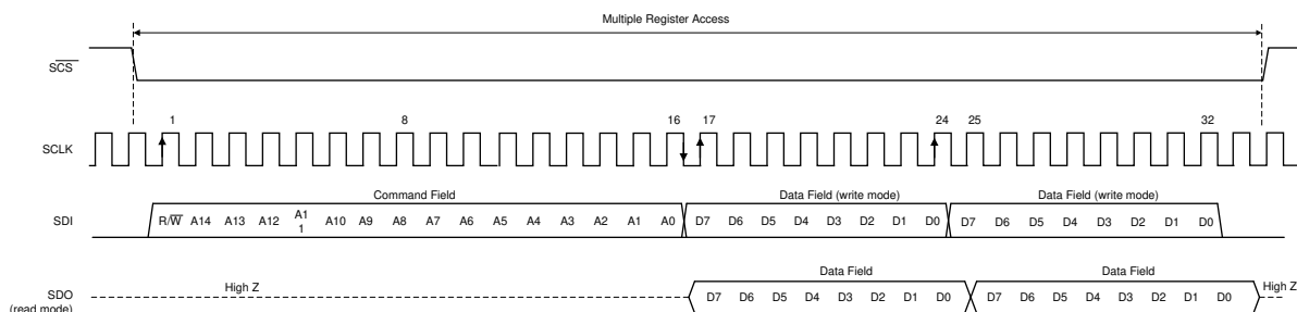
图 7-16. Serial Interface Protocol: Streaming Read/Write
