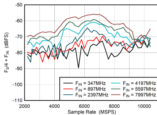
图 6-42. DES Mode: F_S/4 + F_{\text{IN}} vs Sample Rate
