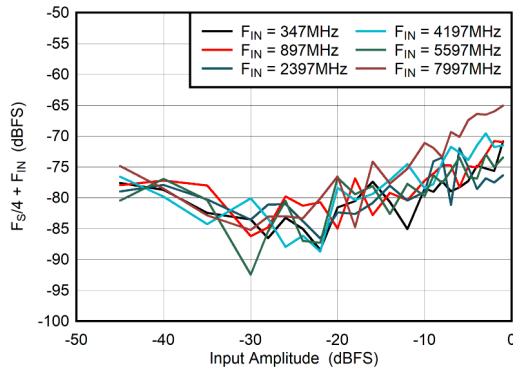
图 6-67. DES Mode: F_S/4 + F_{\text{IN}} vs Input Amplitude
