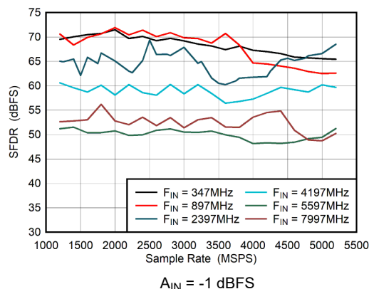
图 6-47. Dual Channel Mode: SFDR vs Sample Rate
