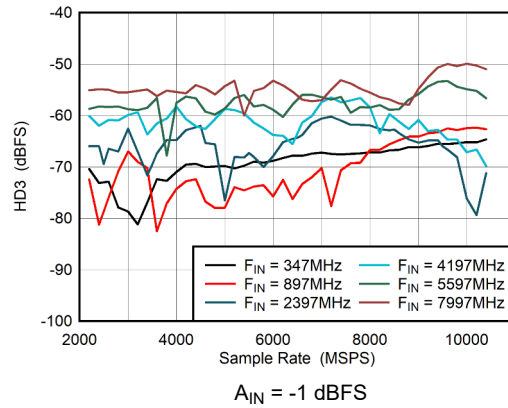
图 6-38. DES Mode: HD3 vs Sample Rate
