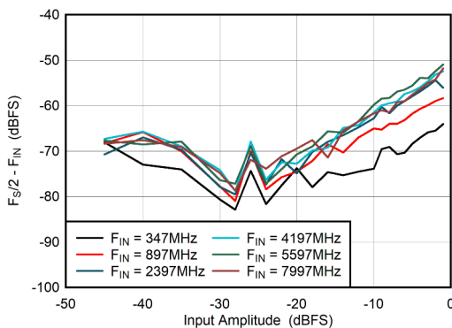
图 6-65. DES Mode: F_S/2 - F_{\text{IN}} vs Input Amplitude
