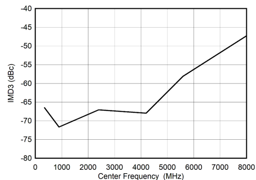
图 6-100. DES Mode: IMD3 vs Input Frequency
