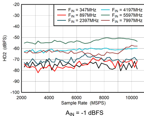
图 6-35. DES Mode: HD2 vs Sample Rate
