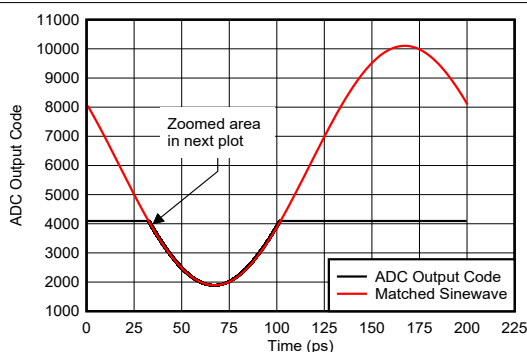
图 6-125. Sinewave Overdrive Recovery
