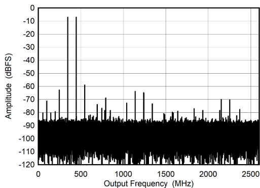
图 6-27. Dual Channel Mode: Two Tone FFT at 5597 MHz
