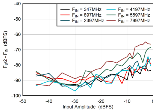
图 6-79. Dual Channel Mode: F_{S/2} - F_{\text{IN}} vs Input Amplitude
