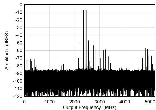
图 6-16. DES Mode: Two Tone FFT at 7997 MHz
