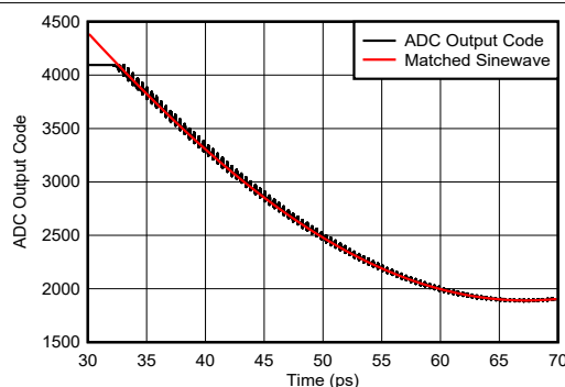
图 6-126. Sinewave Overdrive Recovery
