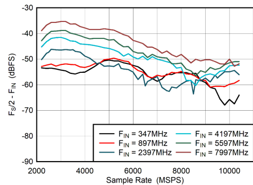
图 6-41. DES Mode: F_S/2 - F_{\text{IN}} vs Sample Rate
