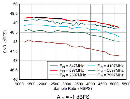
图 6-44. Dual Channel Mode: SNR vs Sample Rate
