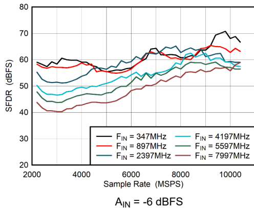
图 6-33. DES Mode: SFDR vs Sample Rate
