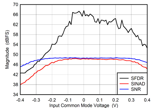
图 6-98. DES Mode: SNR, SFDR and SINAD vs Input Common Mode Voltage
