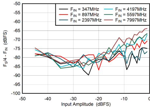
图 6-69. DES Mode: F_S/4 - F_{\text{IN}} vs Input Amplitude
