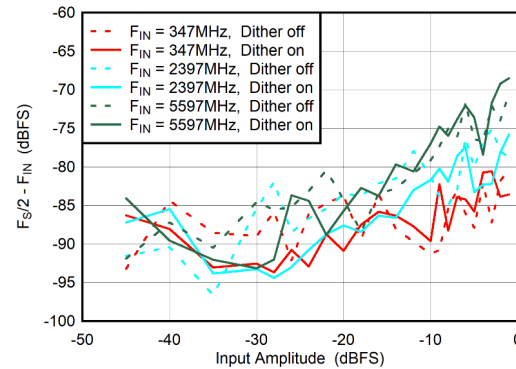
图 6-80. Dual Channel Mode: F_{S/2} - F_{\text{IN}} vs Input Amplitude and Dither
