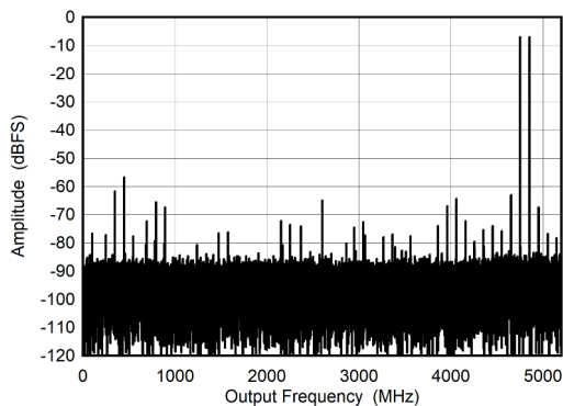
图 6-15. DES Mode: Two Tone FFT at 5597 MHz
