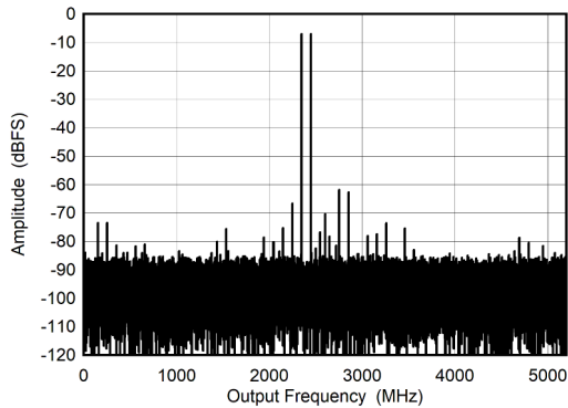
图 6-13. DES Mode: Two Tone FFT at 2397 MHz
