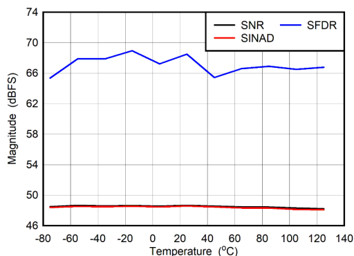
图 6-89. Dual Channel Mode: SNR, SINAD and SFDR vs Temperature
