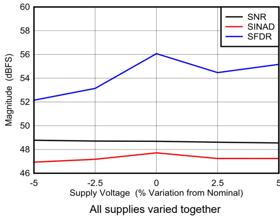
图 6-93. DES Mode: SNR, SINAD and SFDR vs Supply Voltage
