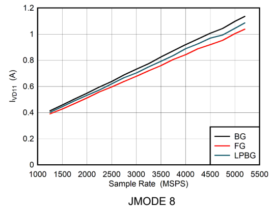
图 6-116. Dual Channel Mode: I_{VD11} vs Sample Rate
