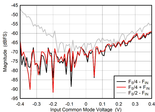
图 6-99. DES Mode: F_S/2 - F_{\text{IN}} , F_S/4 \pm F_{\text{IN}} vs Input Common Mode Voltage
