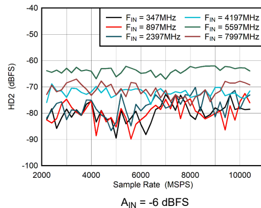
图 6-36. DES Mode: HD2 vs Sample Rate
