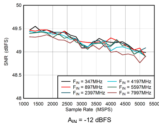
图 6-46. Dual Channel Mode: SNR vs Sample Rate
