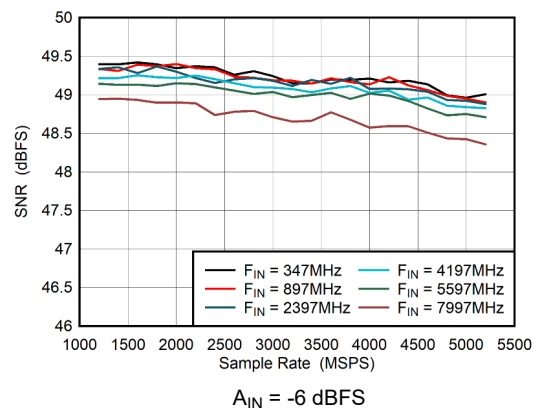
图 6-45. Dual Channel Mode: SNR vs Sample Rate
