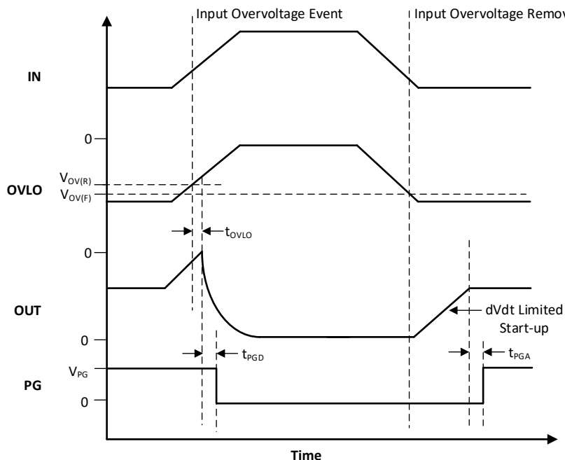
图 8-7. TPS25947x Overvoltage Lockout and Recovery
