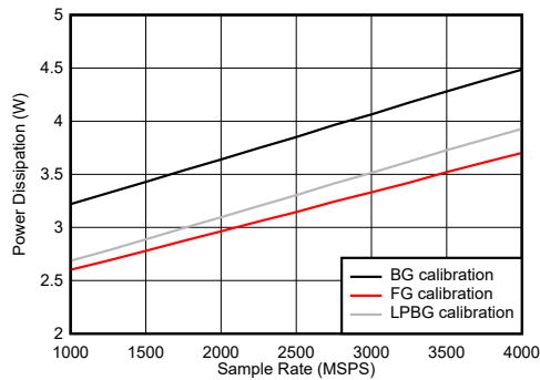
图 7-132. Dual Channel Mode: Power Dissipation vs Sample Rate
