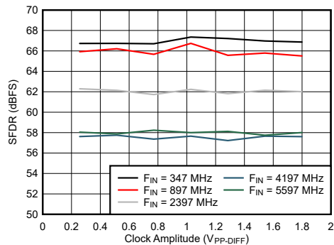
图 7-89. DES Mode: SFDR vs Clock Amplitude
