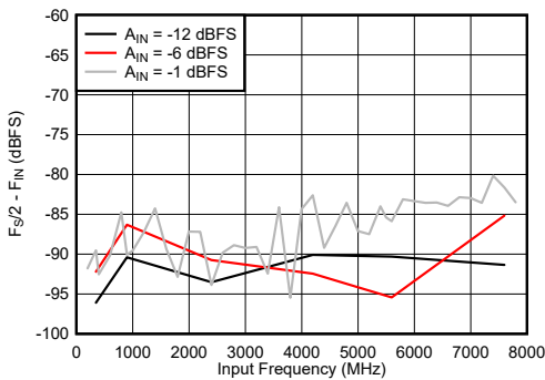
图 7-87. Dual Channel Mode: F_S/2 - F_{\text{IN}} vs Input Frequency
