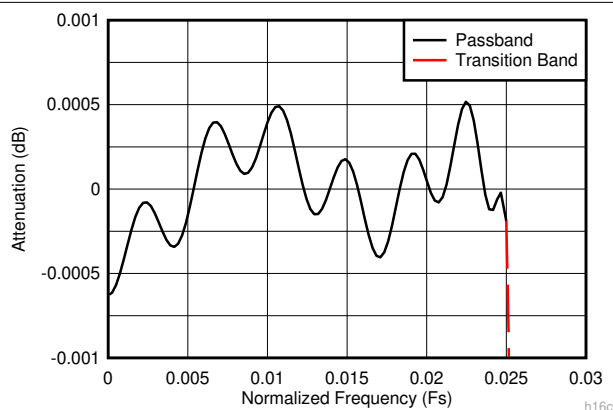
图 8-16. Decimate-by-16 Composite Zoomed Pass-Band Response
