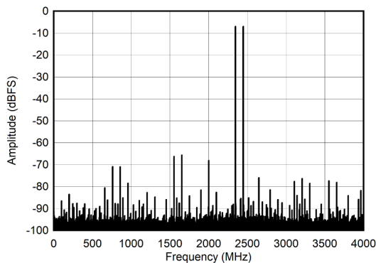
图 7-15. DES Mode: Two Tone FFT at 2397 MHz
