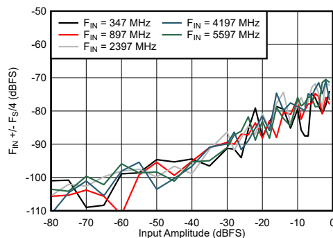
图 7-65. DES Mode: F_{\text{IN}} \pm F_{\text{IN}}/4 vs Input Amplitude and Frequency
