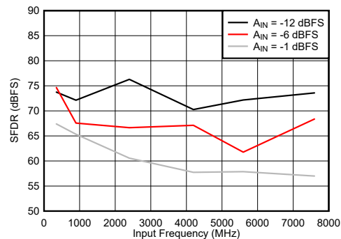
图 7-78. DES Mode: SFDR vs Input Frequency
