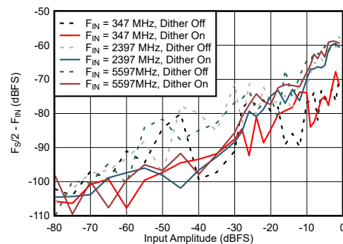
图 7-64. DES Mode: F_{S/2} - F_{\text{IN}} vs Input Amplitude and Dither
