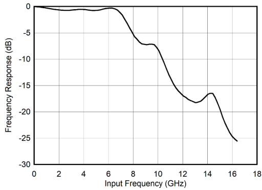
图 7-1. DES Mode: Input Amplitude vs Input Frequency
