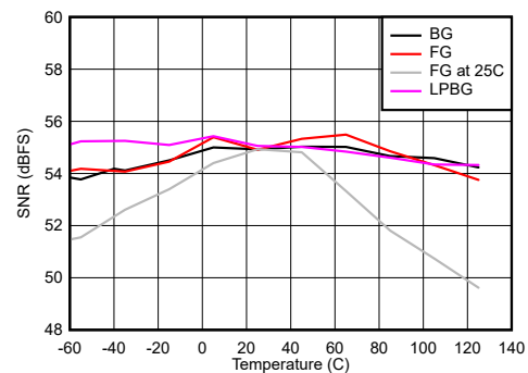
图 7-94. Dual Channel Mode: SNR, SINAD and SFDR vs Temperature
