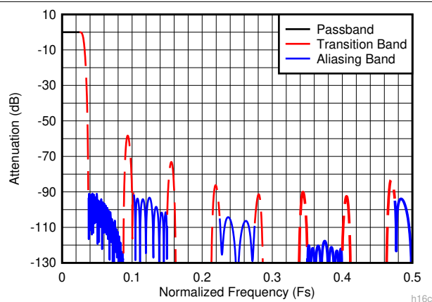
图 8-15. Decimate-by-16 Composite Response
