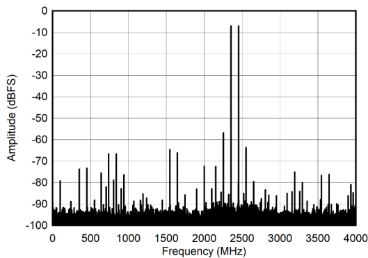
图 7-17. DES Mode: Two Tone FFT at 5597 MHz
