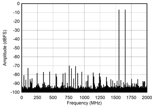
图 7-25. Dual Channel Mode: Two Tone FFT at 2397 MHz
