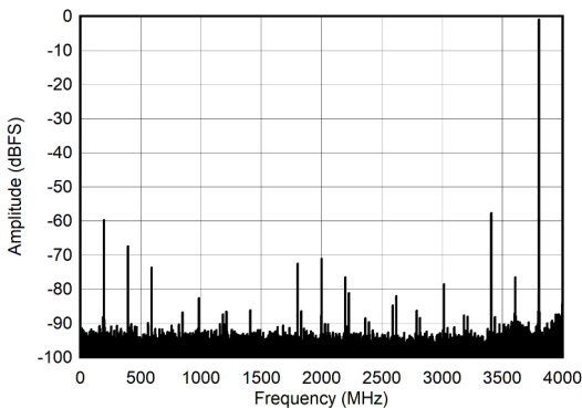
图 7-11. DES Mode: Single Tone FFT at 4197 MHz
