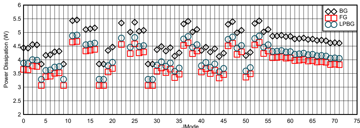
图 7-114. Power Dissipation vs JMODE at F_{\text{CLK}} = 4\text{ GHz}
