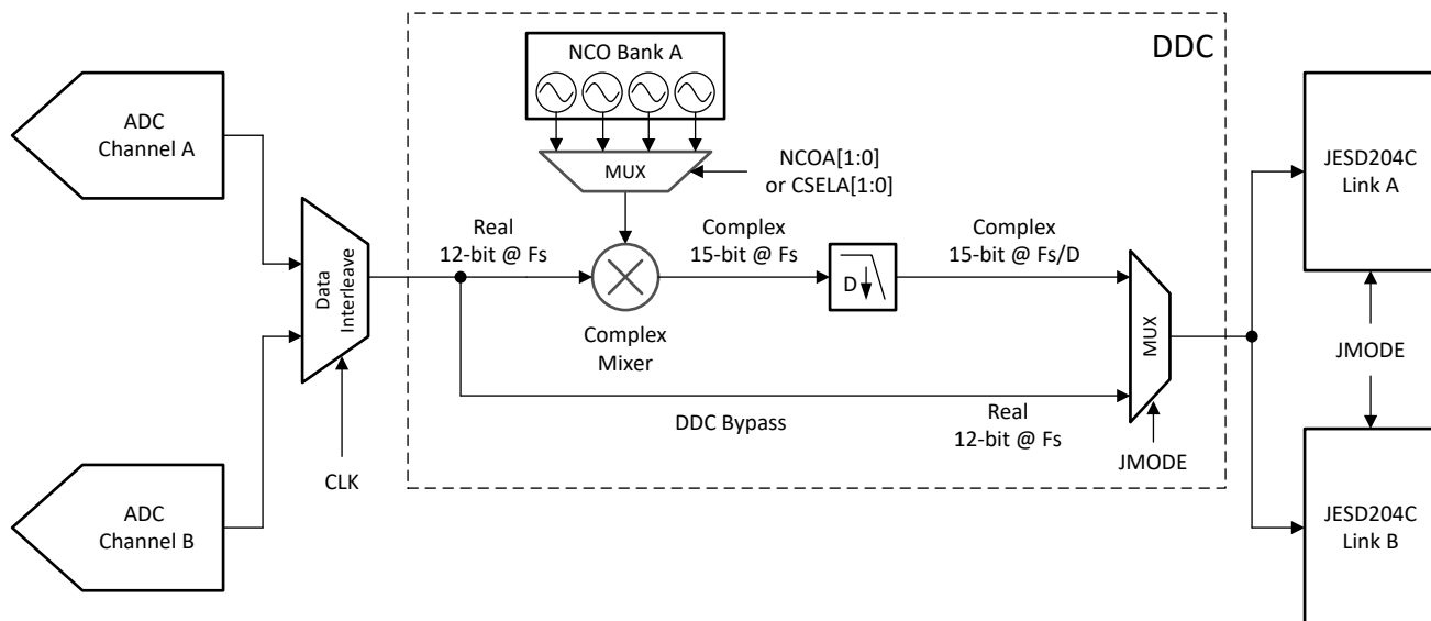
图 8-9. Digital Down Conversion Block in Single Channel Mode
