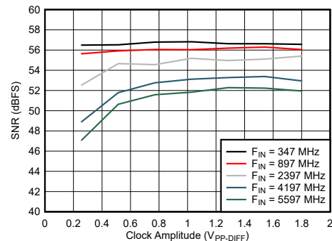
图 7-88. DES Mode: SNR vs Clock Amplitude
