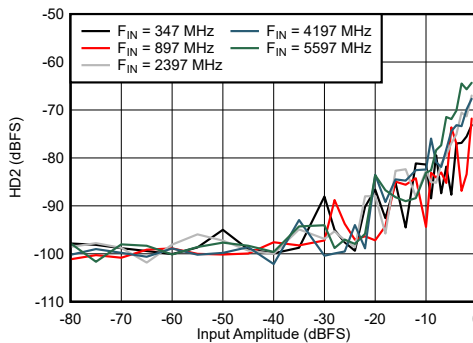
图 7-59. DES Mode: HD2 vs Input Amplitude and Frequency
