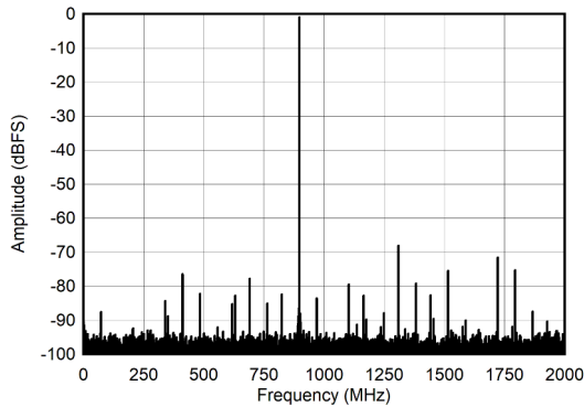
图 7-19. Dual Channel Mode: Single Tone FFT at 897 MHz
