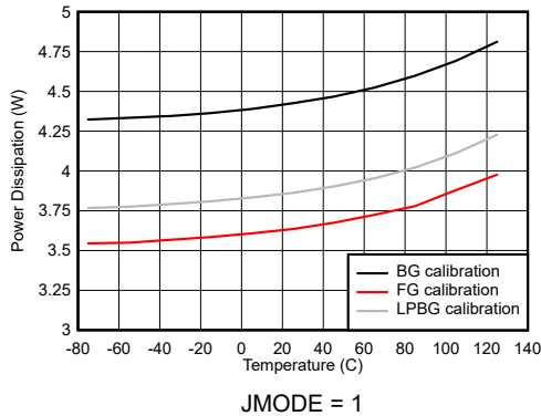
图 7-136. DES Mode: Power Dissipation vs Temperature
