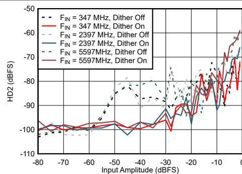
图 7-72. Dual Channel Mode: HD2 vs Input Amplitude and Dither
