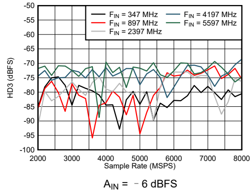
图 7-38. DES Mode: HD3 vs Sample Rate and Input Frequency
