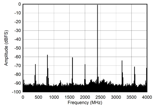
图 7-12. DES Mode: Single Tone FFT at 5597 MHz
