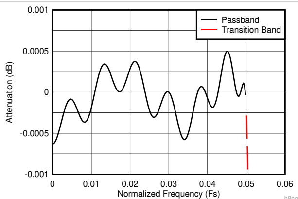
图 8-14. Decimate-by-8 Composite Zoomed Pass-Band Response
