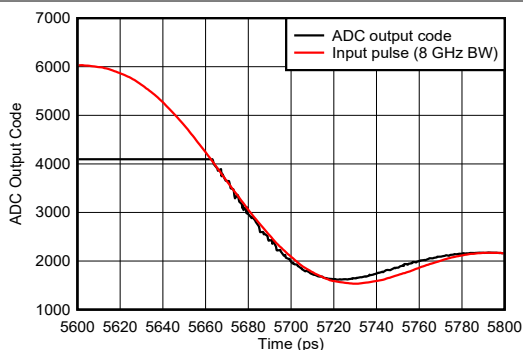
图 7-142. Pulse Overdrive Recovery Zoomed
