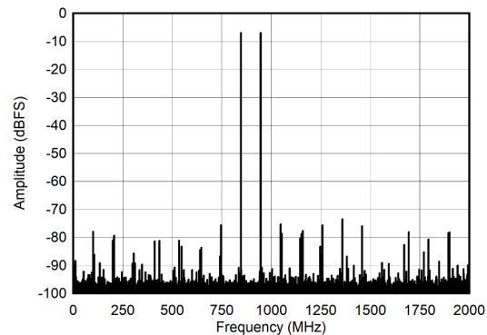
图 7-24. Dual Channel Mode: Two Tone FFT at 897 MHz
