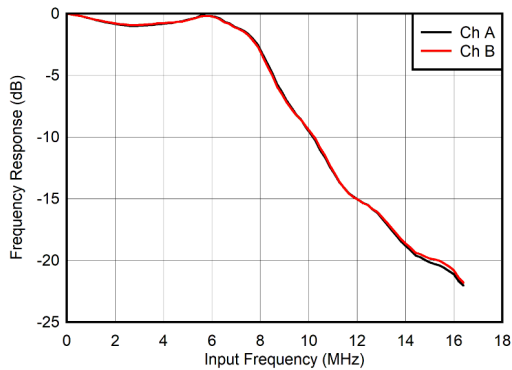
图 7-3. Dual Channel Mode: Input Amplitude vs Input Frequency
