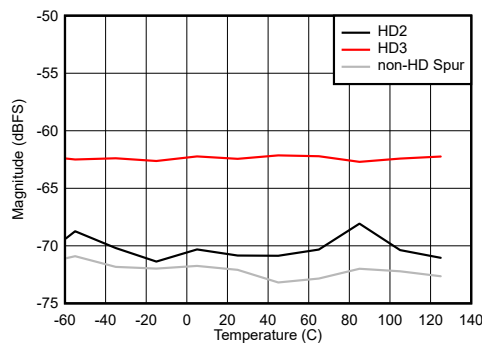
图 7-93. DES Mode: HD2, HD3 and Worst non-HD Spur vs Temperature
