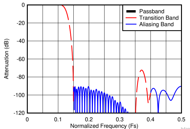
图 8-11. Decimate-by-4 Composite Response
