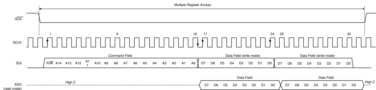
图 8-28. Serial Interface Protocol: Streaming Read/Write
