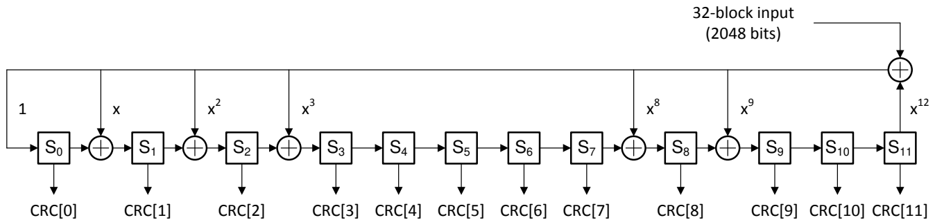
图 8-21. CRC-12 Parity Bit Generator
