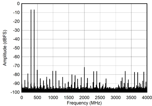
图 7-13. DES Mode: Two Tone FFT at 347 MHz
