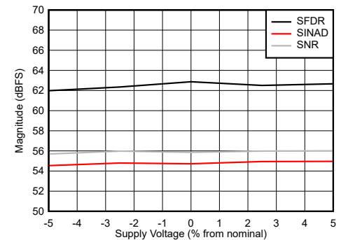
图 7-102. Dual Channel Mode: SNR, SINAD and SFDR vs Supply Voltage
