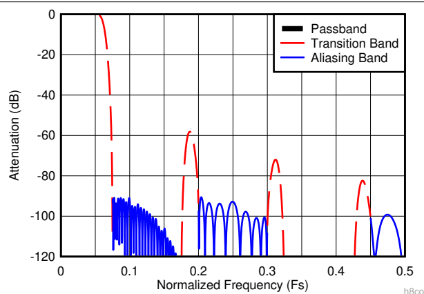
图 8-13. Decimate-by-8 Composite Response
