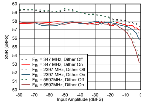
图 7-56. DES Mode: SNR vs Input Amplitude and Dither
