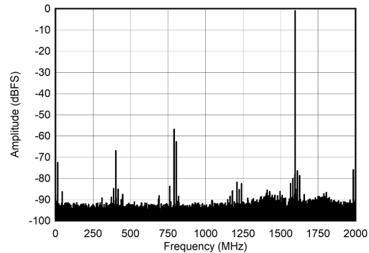
图 7-22. Dual Channel Mode: Single Tone FFT at 5597 MHz
