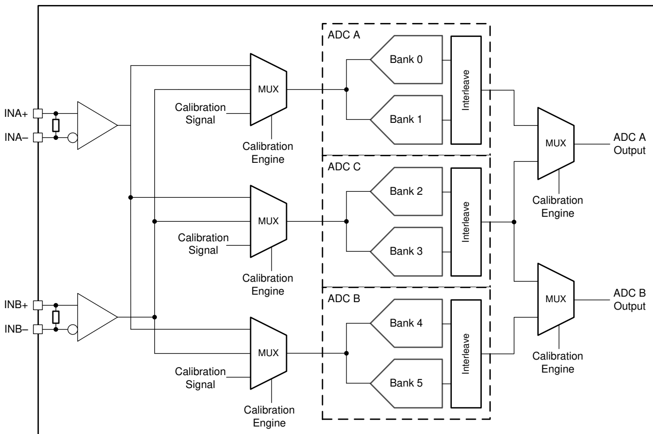
图 8-26. ADC12DJ4000RF Calibration System Block Diagram
