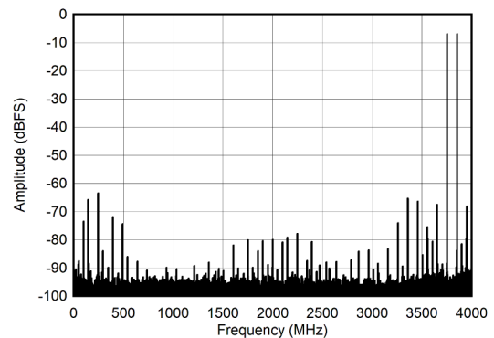
图 7-16. DES Mode: Two Tone FFT at 4197 MHz
