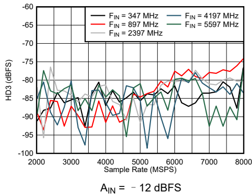
图 7-39. DES Mode: HD3 vs Sample Rate and Input Frequency
