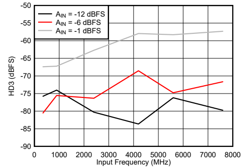
图 7-80. DES Mode: HD3 vs Input Frequency
