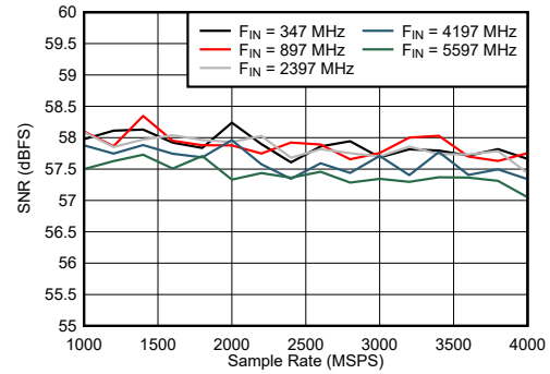
图 7-44. Dual Channel Mode: SNR vs Sample Rate and Input Frequency
