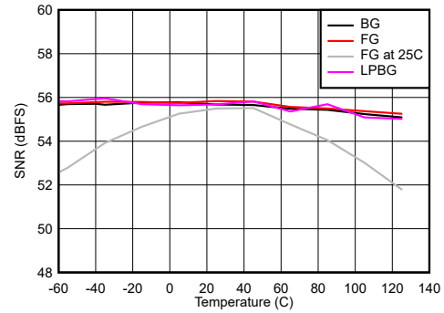
图 7-98. Dual Channel Mode: SNR vs Temperature and Calibration Mode
