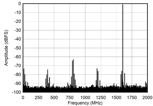
图 7-20. Dual Channel Mode: Single Tone FFT at 2397 MHz
