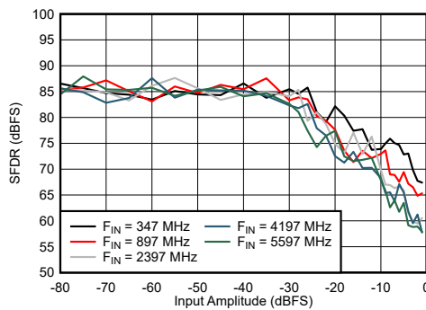
图 7-57. DES Mode: SFDR vs Input Amplitude and Frequency
