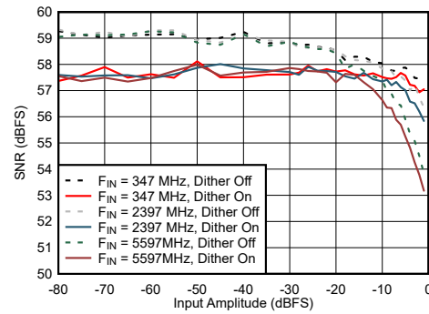
图 7-68. Dual Channel Mode: SNR vs Input Amplitude and Dither
