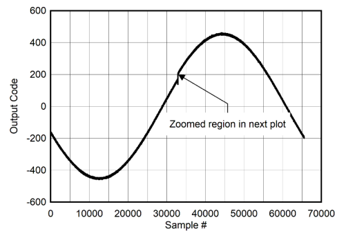
图 7-139. Background Calibration Core Transition (AC Signal)
