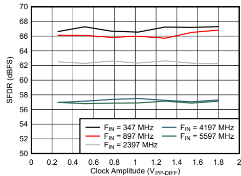
图 7-91. Dual Channel Mode: SFDR vs Clock Amplitude
