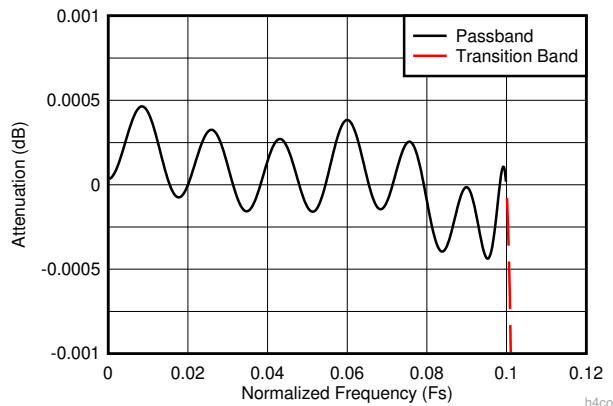
图 8-12. Decimate-by-4 Composite Zoomed Pass-Band Response
