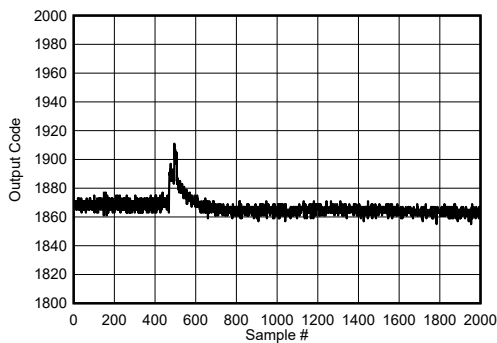
图 7-138. Background Calibration Core Transition (DC Offset Signal)
