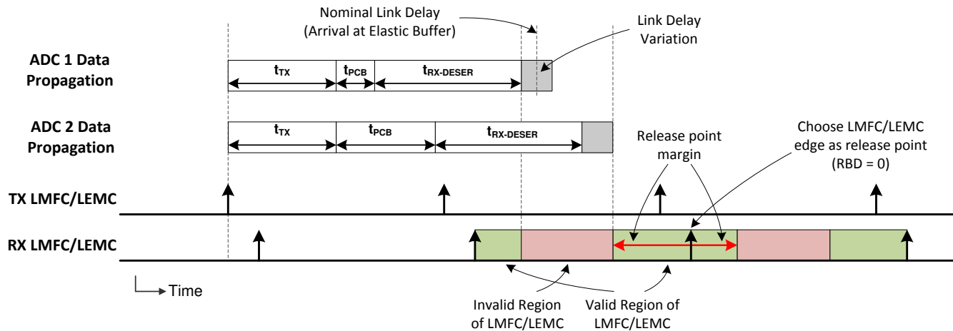
图 8-23. LMFC/LEMC Valid Region Definition for Elastic Buffer Release Point Selection
