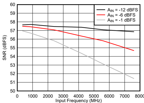
图 7-77. DES Mode: SNR vs Input Frequency
