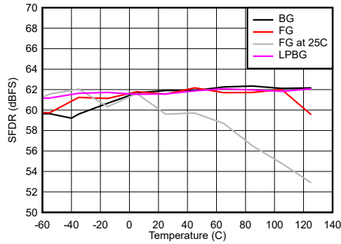
图 7-97. DES Mode: SFDR vs Temperature and Calibration Mode
