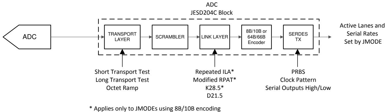
图 8-25. Test Mode Insertion Points
