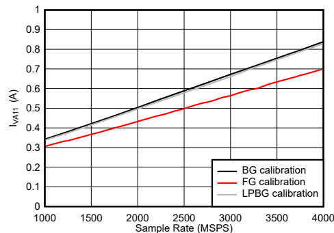
图 7-117. DES Mode: I_{V_{A11}} vs Sample Rate
