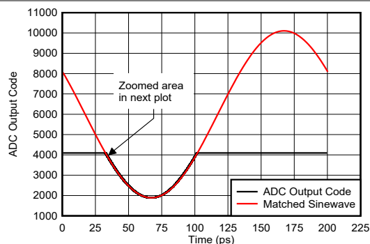
图 7-143. Sinewave Overdrive Recovery
