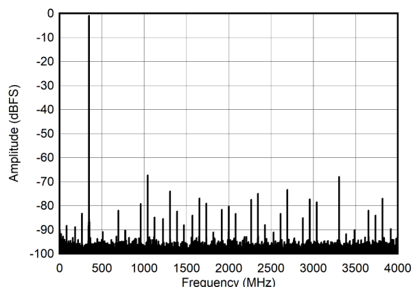
图 9-2. FFT for 347 MHz Input Signal, 8 GSPS, JMODE1
