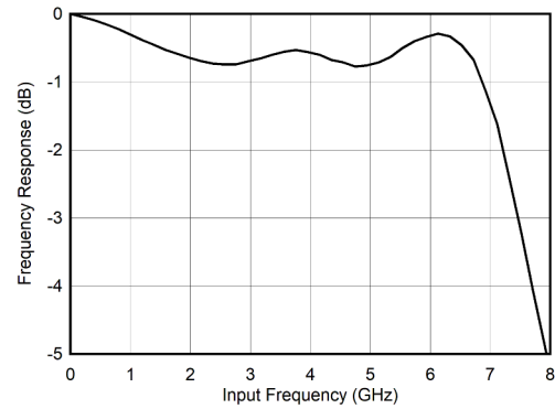
图 7-2. DES Mode: Input Response vs Input Frequency
