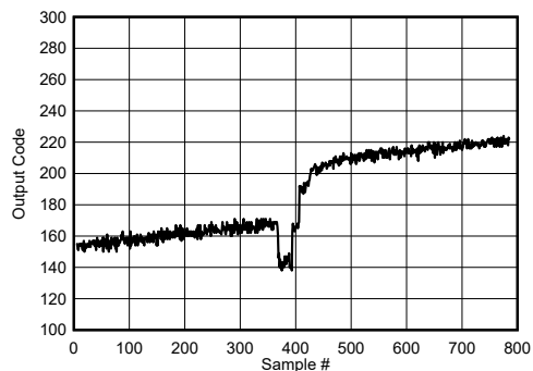
图 7-140. Background Calibration Core Transition (AC Signal Zoomed)
