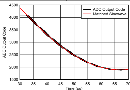
图 7-144. Sinewave Overdrive Recovery
