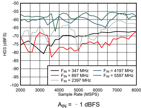
图 7-37. DES Mode: HD3 vs Sample Rate and Input Frequency
