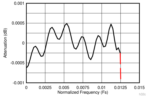
图 8-18. Decimate-by-32 Composite Zoomed Pass-Band Response
