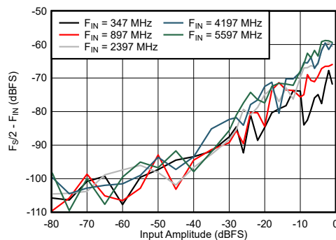
图 7-63. DES Mode: F_{S/2} - F_{\text{IN}} vs Input Amplitude and Frequency
