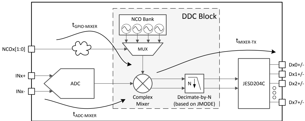
图 8-10. NCO Fast Frequency Hopping Latency Diagram
