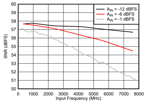
图 7-83. Dual Channel Mode: SNR vs Input Frequency
