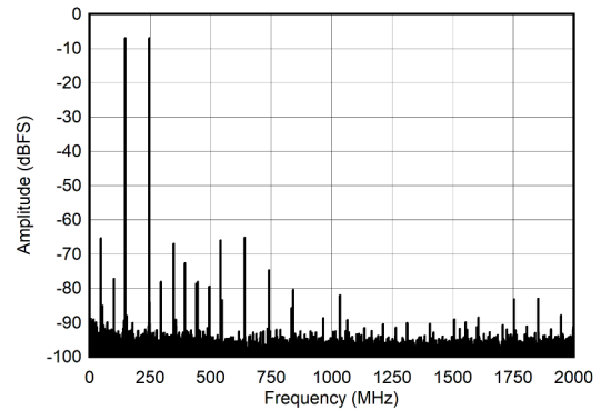
图 7-26. Dual Channel Mode: Two Tone FFT at 4197 MHz
