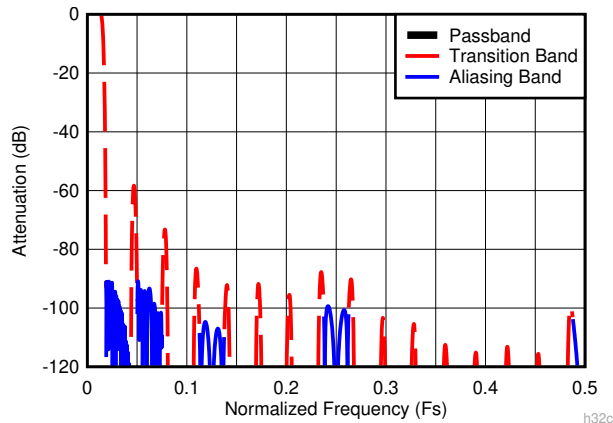
图 8-17. Decimate-by-32 Composite Response
