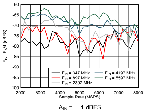
图 7-41. DES Mode: F_{\text{IN}} \pm F_{S/4} vs Sample Rate and Input Frequency
