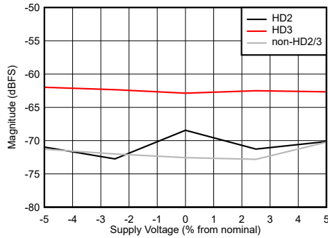
图 7-103. Dual Channel Mode: HD2, HD3 and Worst non-HD Spur vs Supply Voltage
