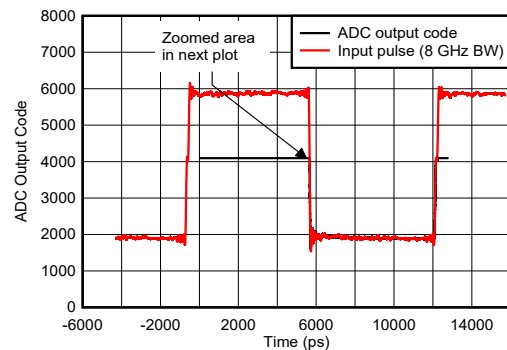
图 7-141. Pulse Overdrive Recovery
