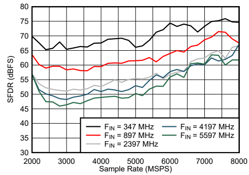
图 7-32. DES Mode: SFDR vs Sample Rate and Input Frequency
