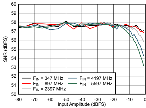
图 7-67. Dual Channel Mode: SNR vs Input Amplitude and Frequency
