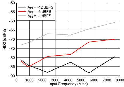
图 7-79. DES Mode: HD2 vs Input Frequency
