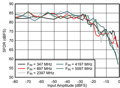
图 7-69. Dual Channel Mode: SFDR vs Input Amplitude and Frequency
