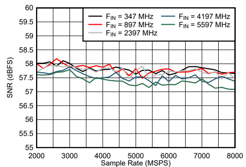
图 7-30. DES Mode: SNR vs Sample Rate and Input Frequency
