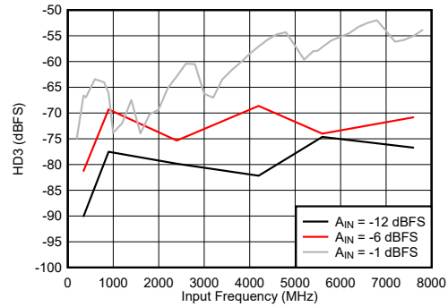
图 7-86. Dual Channel Mode: HD3 vs Input Frequency
