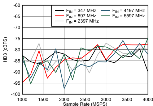
图 7-51. Dual Channel Mode: HD3 vs Sample Rate and Input Frequency
