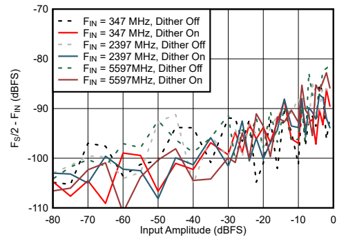
图 7-76. Dual Channel Mode: F_S/2 - F_{\text{IN}} vs Input Amplitude and Dither
