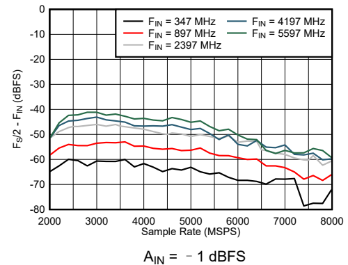
图 7-40. DES Mode: F_{S/2} - F_{\text{IN}} vs Sample Rate and Input Frequency
