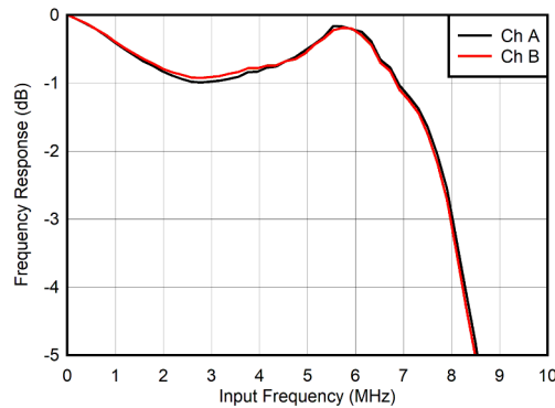
图 7-4. Input Response vs Input Frequency (zoomed)
