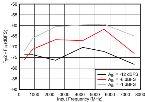
图 7-81. DES Mode: F_s/2 - F_{\text{IN}} vs Input Frequency
