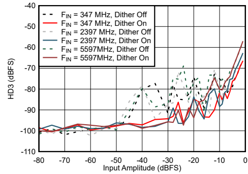
图 7-74. Dual Channel Mode: HD3 vs Input Amplitude and Dither
