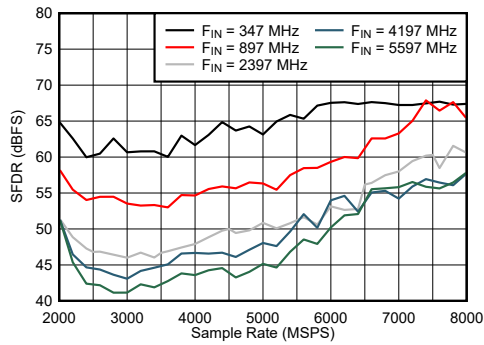
图 7-31. DES Mode: SFDR vs Sample Rate and Input Frequency
