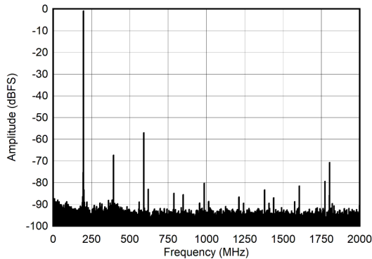
图 7-21. Dual Channel Mode: Single Tone FFT at 4197 MHz
