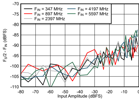
图 7-75. Dual Channel Mode: F_S/2 - F_{\text{IN}} vs Input Amplitude and Frequency
