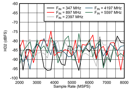
图 7-34. DES Mode: HD2 vs Sample Rate and Input Frequency
