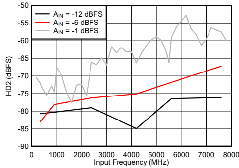
图 7-85. Dual Channel Mode: HD2 vs Input Frequency
