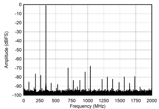
图 7-18. Dual Channel Mode: Single Tone FFT at 347 MHz
