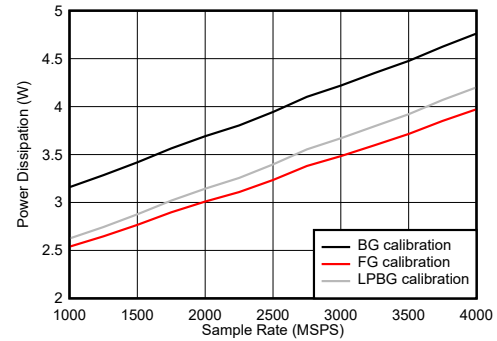
图 7-125. DES Mode: Power Dissipation vs Sample Rate
