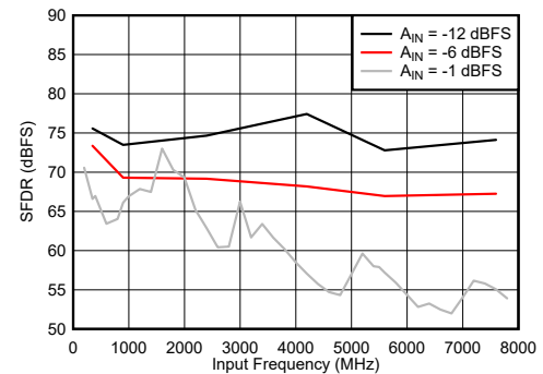
图 7-84. Dual Channel Mode: SFDR vs Input Frequency
