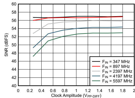
图 7-90. Dual Channel Mode: SNR vs Clock Amplitude
