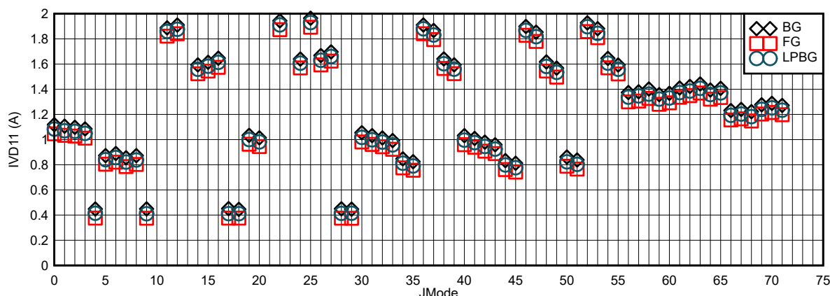
图 7-115. I_{V_{D11}} vs JMODE at F_{\text{CLK}} = 4\text{ GHz}
