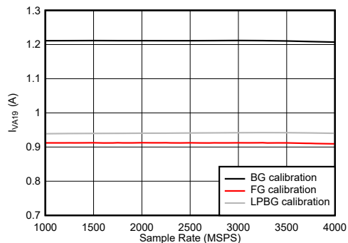
图 7-116. DES Mode: I_{V_{A19}} vs Sample Rate
