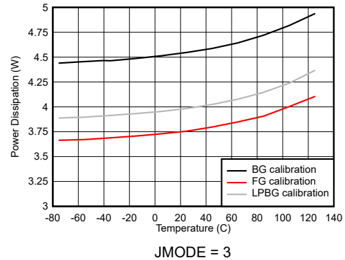
图 7-137. Dual Channel Mode: Power Dissipation vs Temperature
