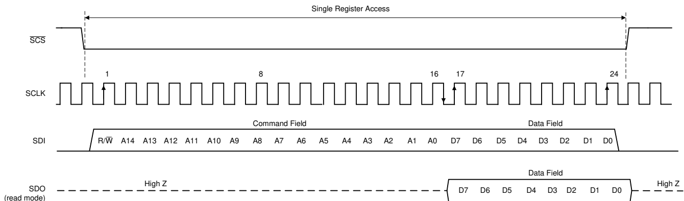
图 8-27. Serial Interface Protocol: Single Read/Write
