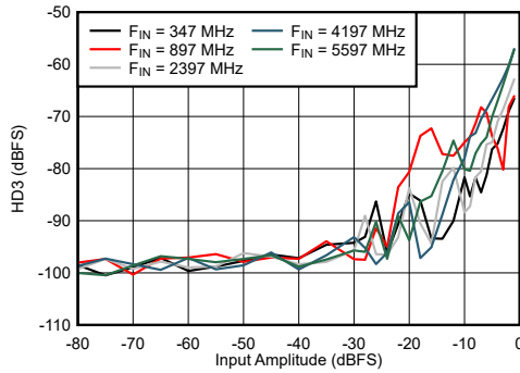
图 7-73. Dual Channel Mode: HD3 vs Input Amplitude and Frequency
