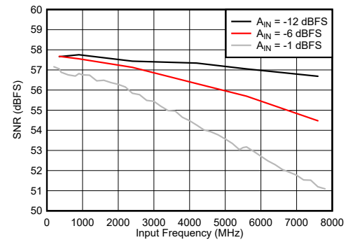
图 7-82. DES Mode: F_{\text{IN}} \pm F_s/4 vs Input Frequency
