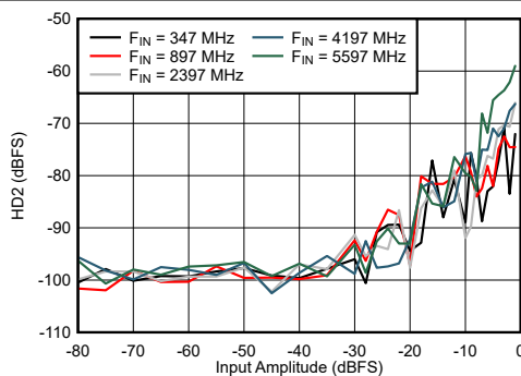
图 7-71. Dual Channel Mode: HD2 vs Input Amplitude and Frequency
