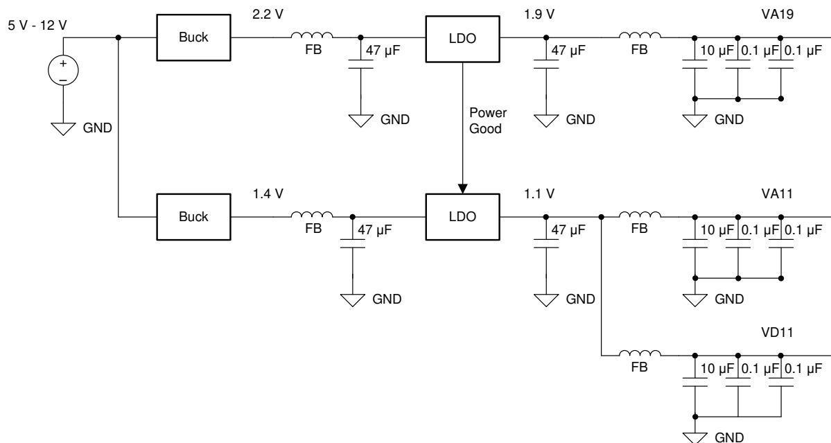
图 10-1. LDO Linear Regulator Approach Example
