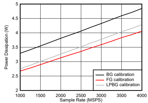
图 7-133. Dual Channel Mode: Power Dissipation vs Sample Rate
