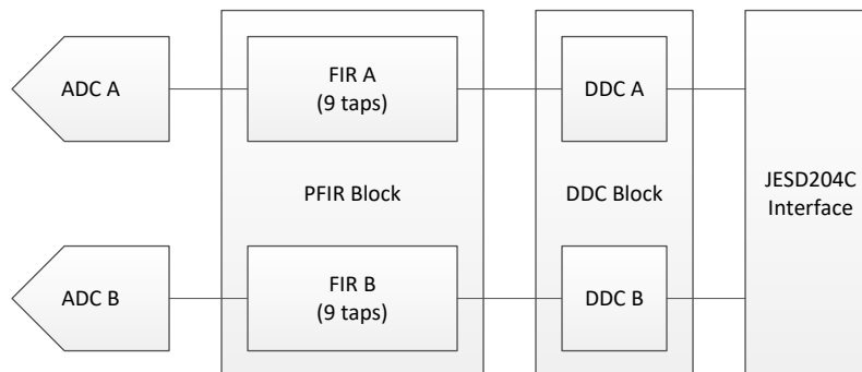
图 8-4. Dual Channel Equalization PFIR Block Diagram
