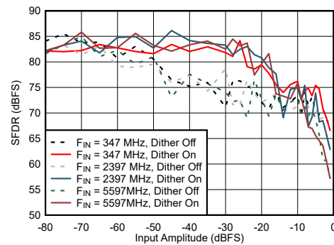
图 7-70. Dual Channel Mode: SFDR vs Input Amplitude and Dither
