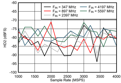
图 7-50. Dual Channel Mode: HD2 vs Sample Rate and Input Frequency
