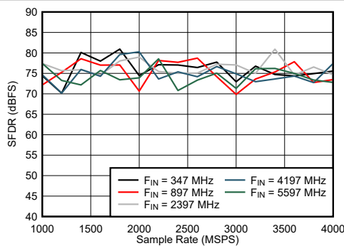
图 7-45. Dual Channel Mode: SFDR vs Sample Rate and Input Frequency
