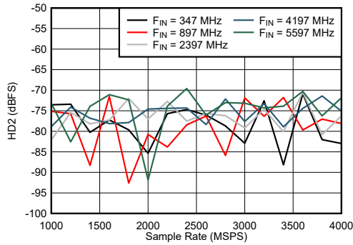
图 7-49. Dual Channel Mode: HD2 vs Sample Rate and Input Frequency
