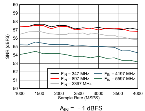
图 7-42. Dual Channel Mode: SNR vs Sample Rate and Input Frequency
