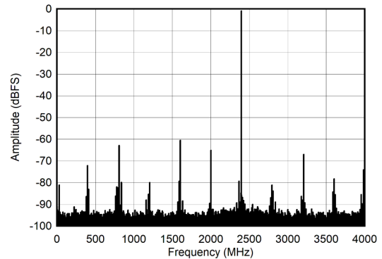
图 7-10. DES Mode: Single Tone FFT at 2397 MHz
