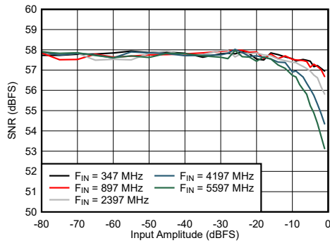
图 7-55. DES Mode: SNR vs Input Amplitude and Frequency
