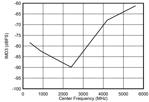
图 7-104. DES Mode: IMD3 vs Input Frequency
