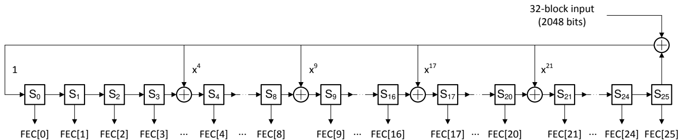
图 8-22. FEC Parity Bit Generator
