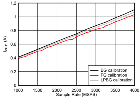
图 7-118. DES Mode: I_{VD11} vs Sample Rate
