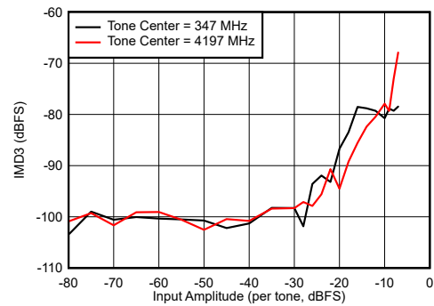
图 7-106. DES Mode: IMD3 vs Input Amplitude
