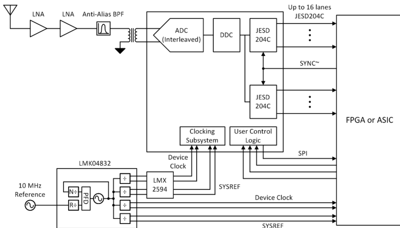
图 9-1. Typical Configuration for Wideband RF Sampling
