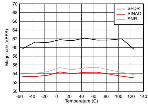
图 7-92. DES Mode: SNR, SINAD and SFDR vs Temperature
