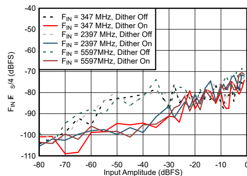
图 7-66. DES Mode: F_{\text{IN}} \pm F_{\text{IN}}/4 vs Input Amplitude and Dither
