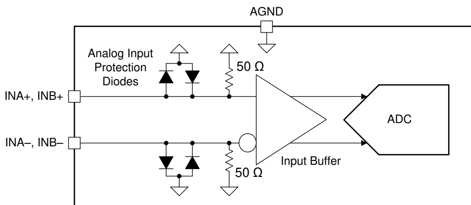
图 8-1. ADC12DJ4000RF Analog Input Internal Termination and Protection Diagram
