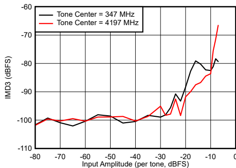
图 7-107. Dual Channel Mode: IMD3 vs Input Amplitude
