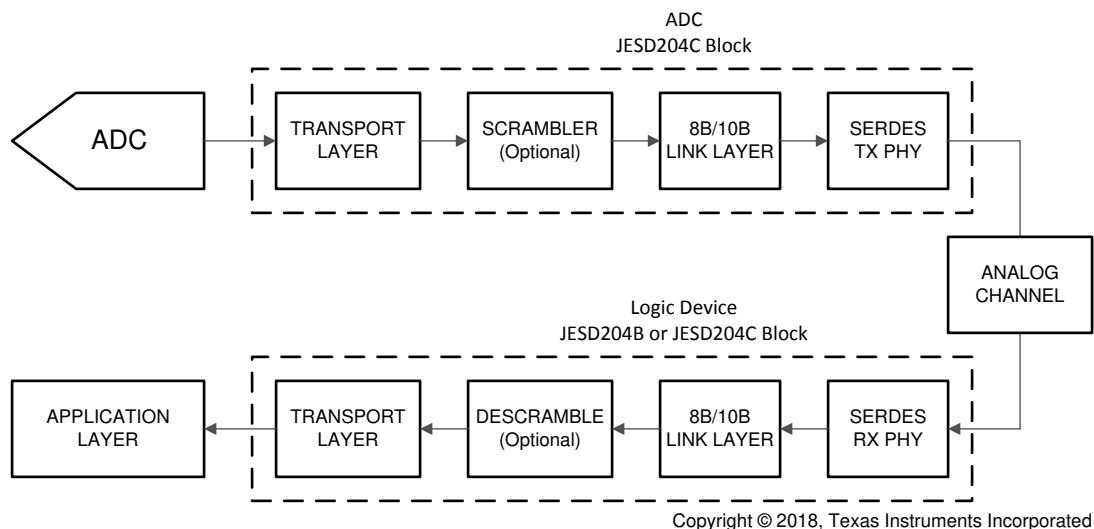
图 8-19. Simplified 8B/10B Encoded JESD204C Interface Diagram
