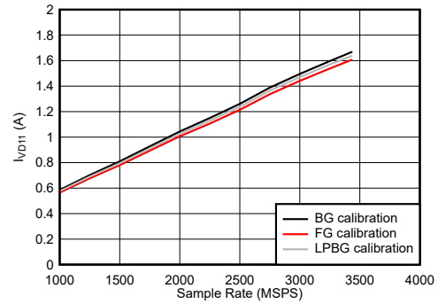
图 7-119. DES Mode: I_{VD11} vs Sample Rate
