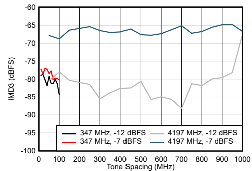
图 7-108. DES Mode: IMD3 vs Tone Spacing
