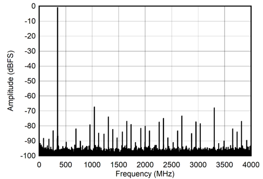
图 7-8. DES Mode: Single Tone FFT at 347 MHz
