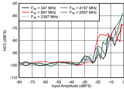
图 7-61. DES Mode: HD3 vs Input Amplitude and Frequency
