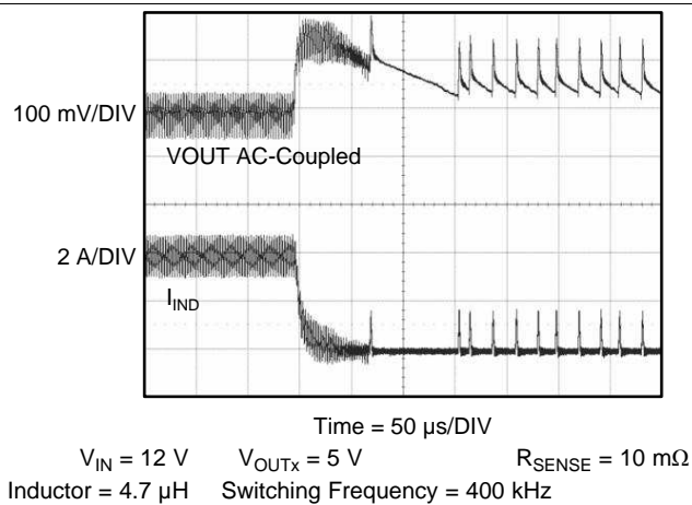
图 5. Buck1 and Buck2 Load Step: Low-Power-Mode Entry (0.09 mA to 4 A at 2.5 A/μs)
