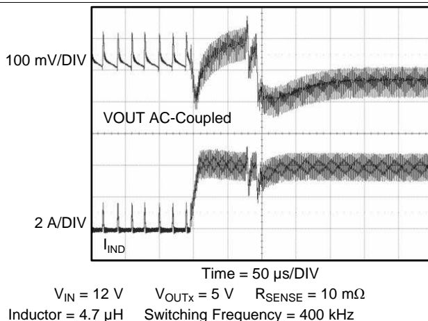
图 6. Buck1 AND Buck2 Load Step: Low-Power-Mode Exit (0.09 mA to 4 A AT 2.5 A/μs)
