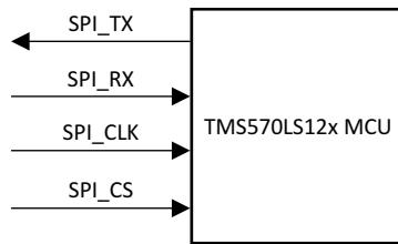
Figure 1. SPI Connections for TMS570LS12x Bootloader
