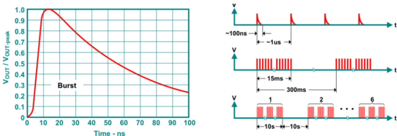
Figure 1. Voltage Waveform of an EFT Pulse and Timing Sequence of an Entire Test Cycle
