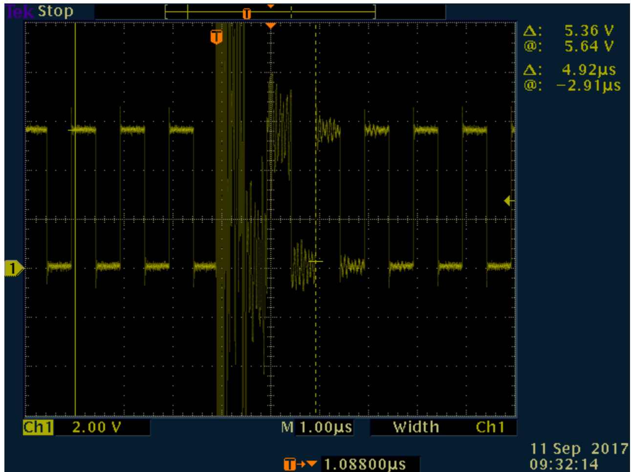
Figure 2. THVD1500 Bus Voltage Waveform During EFT Strike
