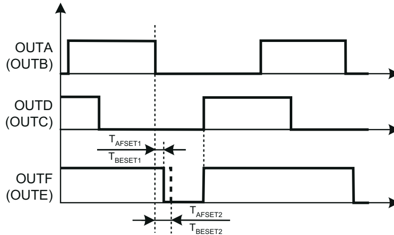
图 7-4. Delay Definitions Between OUTA and OUTF , OUTB and OUE
