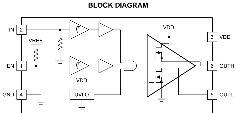
Figure 2. UCC27531-Q1 (EN Pullup Resistance to VREF = 500 kΩ, VREF = 5.8 V, in Pulldown Resistance to GND = 230 kΩ)
