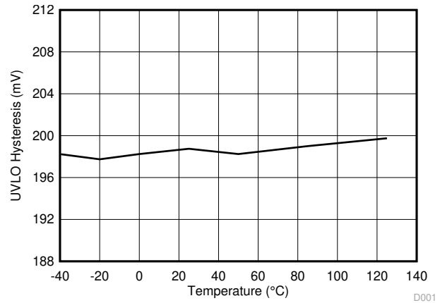
图 5-10. VCCI UVLO Threshold Hysteresis Voltage
