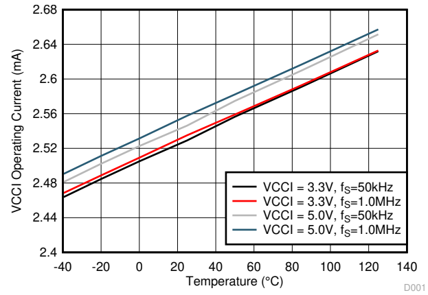
图 5-4. VCCI Operating Current - I_{VCCI}
