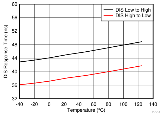
图 5-20. DISABLE Response Time
