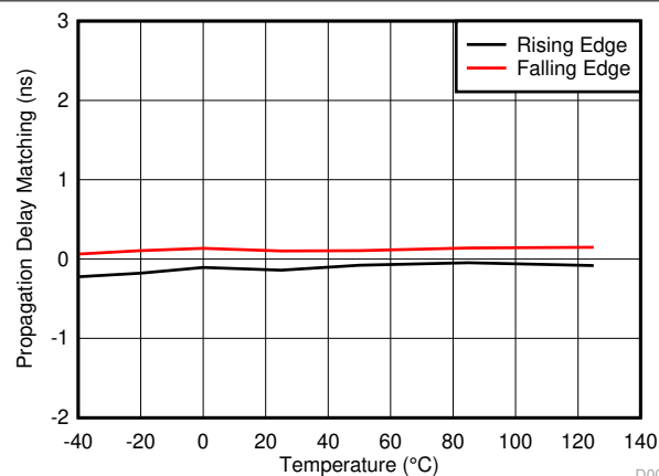
图 5-17. Propagation Delay Matching, Rising and Falling Edge
