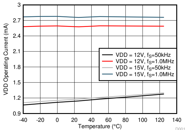
图 5-7. VDD Per Channel Operating Current - I_{VDDA/B}
