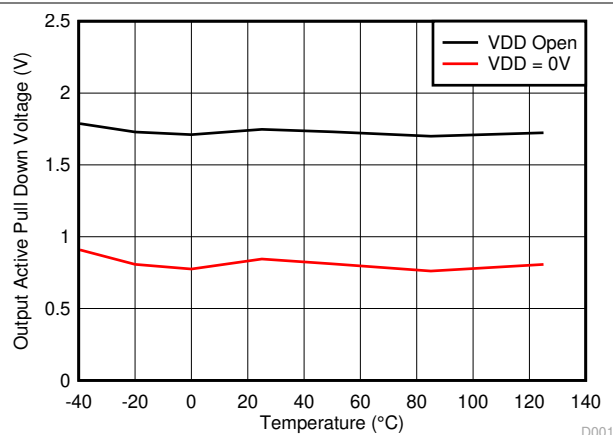
图 5-21. OUTPUT Active Pulldown Voltage
