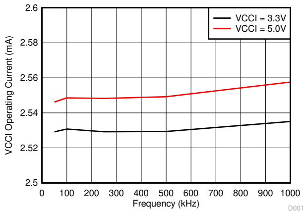
图 5-5. VCCI Operating Current vs. Frequency
