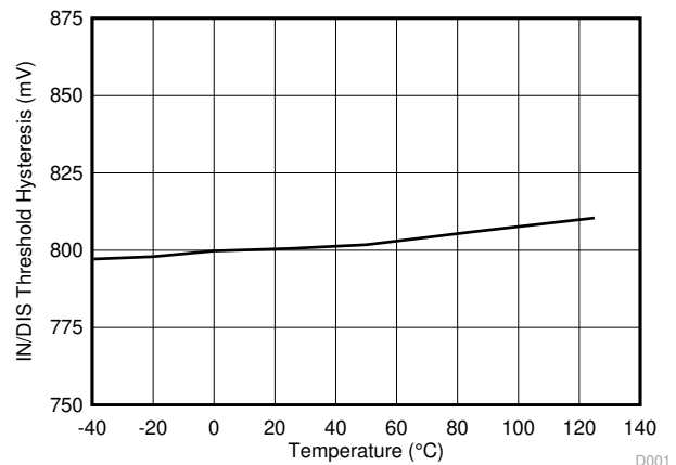
图 5-14. INA/INB/DIS High and Low Threshold Hysteresis
