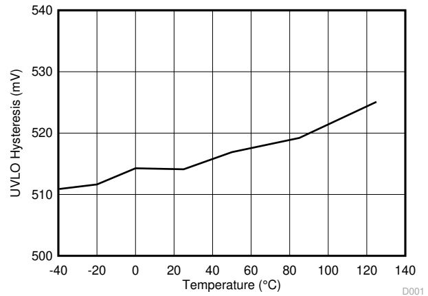
图 5-12. VDD UVLO Threshold Hysteresis Voltage
