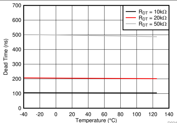
图 5-23. Dead Time Temperature Drift
