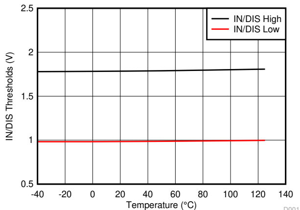
图 5-13. INA/INB/DIS High and Low Threshold Voltage
