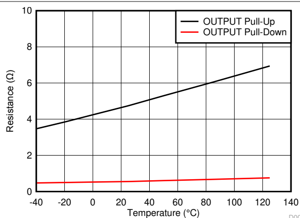
图 5-15. OUT Pullup and Pulldown Resistance
