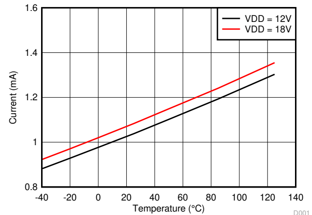
图 5-6. VDD Per Channel Quiescent Current ( I_{VDDA} , I_{VDDB} )
