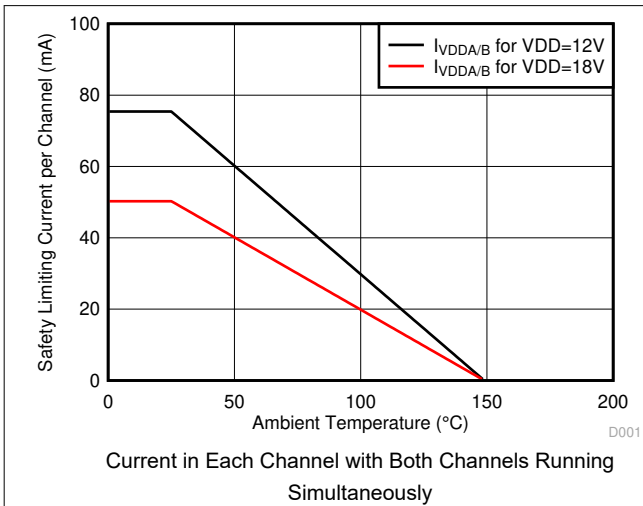
图 5-1. Thermal Derating Curve for Limiting Current Per VDE
