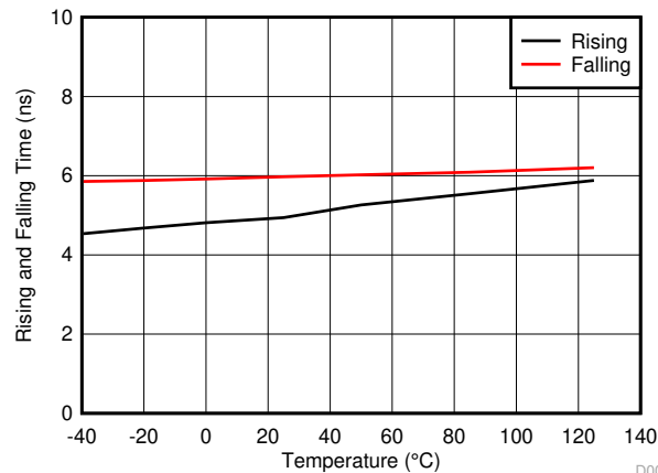
图 5-19. Rise Time and Fall Time
