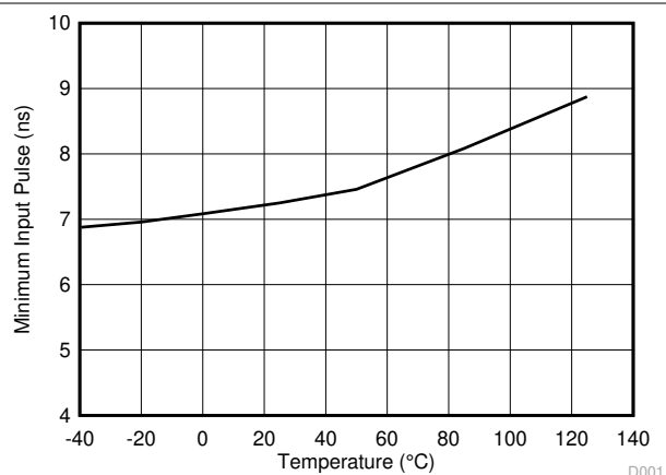
图 5-22. Minimum Pulse that Changes Output
