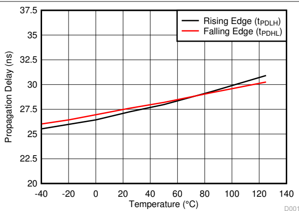
图 5-16. Propagation Delay, Rising and Falling Edge
