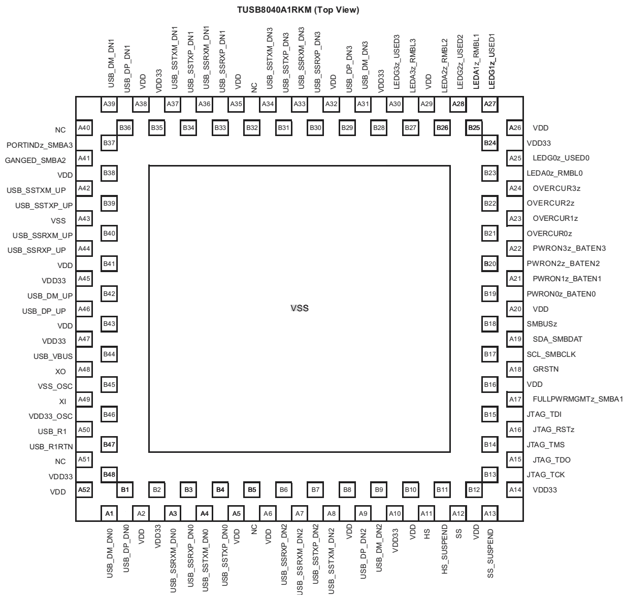
图 5-1. 100-Pin TUSB8040A1 RKM Package, 100-Pin WQFN (Top View)
