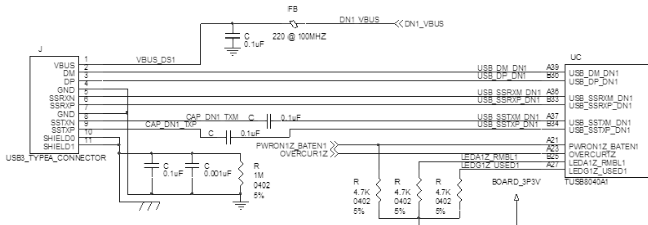
图 8-4. Downstream Port 2 Implementation
