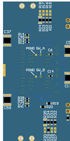
图 7-20. Bottom-Layer Components (Top View)
