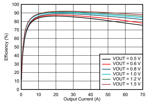
图 5-2. TPSM8D6C24 Efficiency vs Output Current
