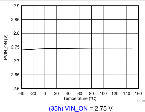
图 5-14. Turn-On Voltage vs Junction Temperature
