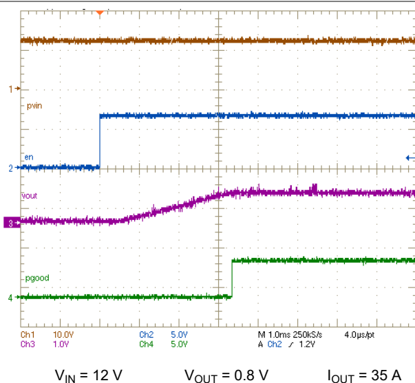
图 7-5. Start-Up from EN/UVLO
