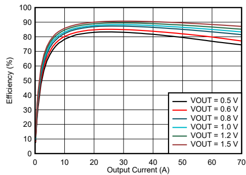
图 5-1. TPSM8D6C24 Efficiency vs Output Current
