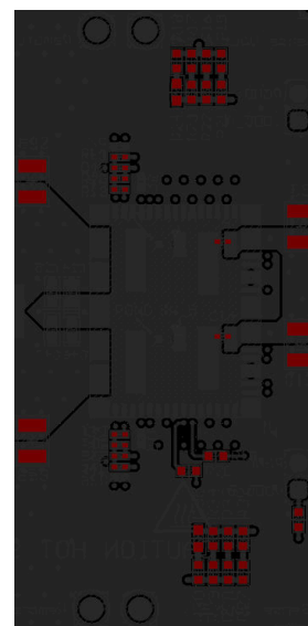
图 7-22. Bottom-Layer Layout (Top View)
