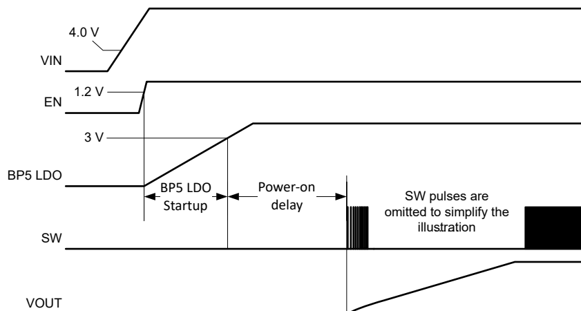
图 6-1. Start-Up Sequence
