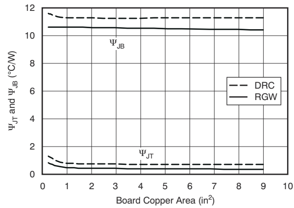
图 8-15. \Psi_{JT} and \Psi_{JB} vs Board Size
