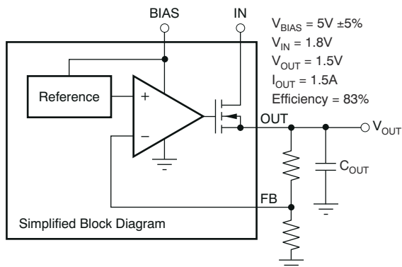
图 8-2. Typical Application of the TPS748 Using an Auxiliary Bias Rail
