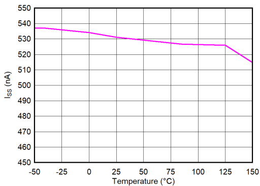
图 6-39. Soft-Start Charging Current ( I_{SS} ) vs Temperature ( T_J )
