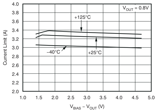
图 8-11. Current Limit vs ( V_{\text{BIAS}} - V_{\text{OUT}} )
