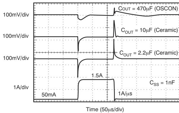
图 8-5. Output Load Transient Response
