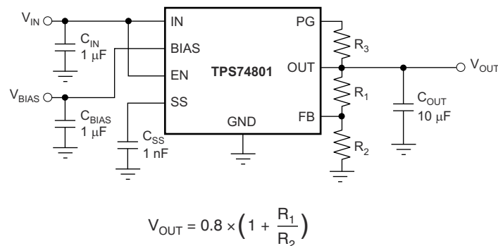
图 8-1. Typical Application Circuit for the TPS748 (Adjustable)
