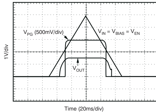
图 8-7. Power-Up, Power-Down
