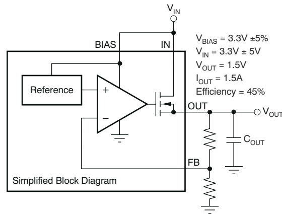
图 8-8. Typical Application of the TPS748 Without an Auxiliary Bias Rail
