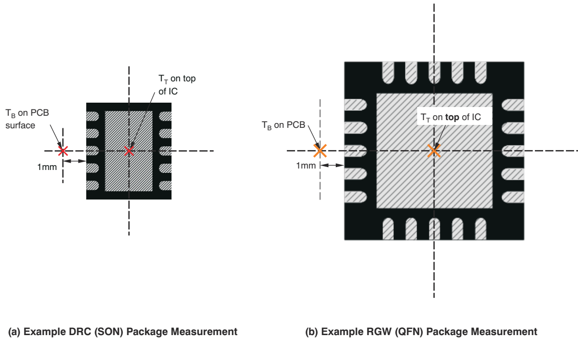
图 8-14. Measuring Points for T_T and T_B
