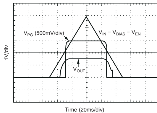
图 6-22. Power-Up, Power-Down
