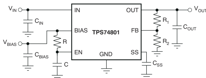
图 7-1. Soft-Start Delay Using an RC Circuit to Enable the Device
