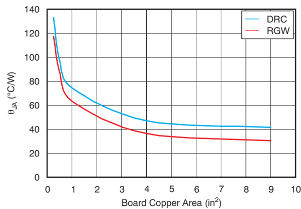
图 8-13. R_{\theta JA} vs Board Size
