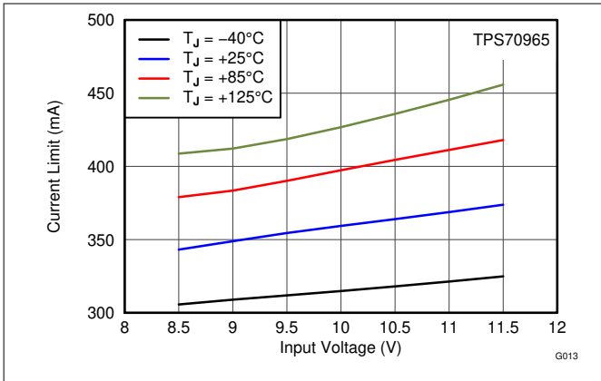
图 6-13. 6.5-V Current Limit vs V_{IN} and Temperature
