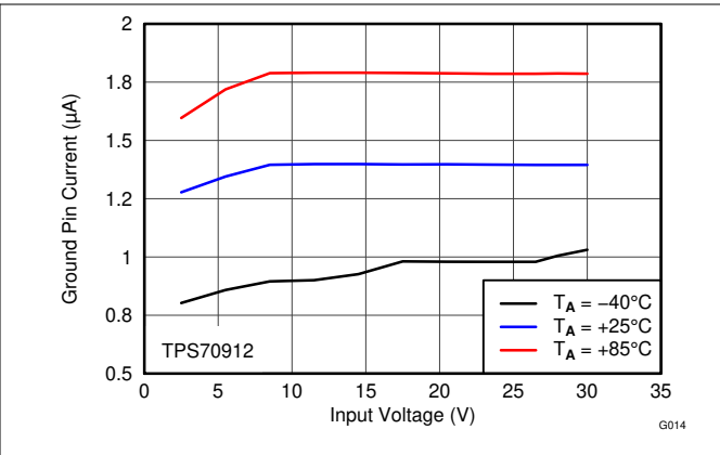
图 6-14. GND Current vs V_{IN} and Temperature
