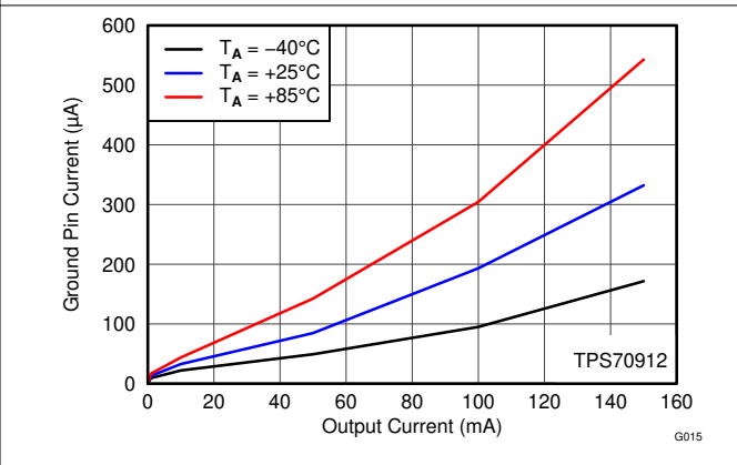
图 6-16. GND Current vs I_{OUT} and Temperature
