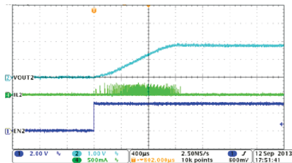
图 8-5. Buck2, Soft-Start With No Load
