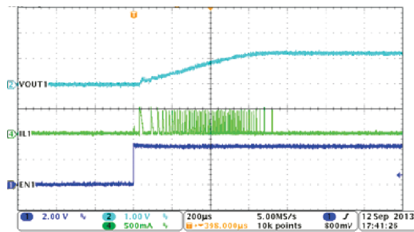
图 8-3. Buck1, Soft-Start With No Load
