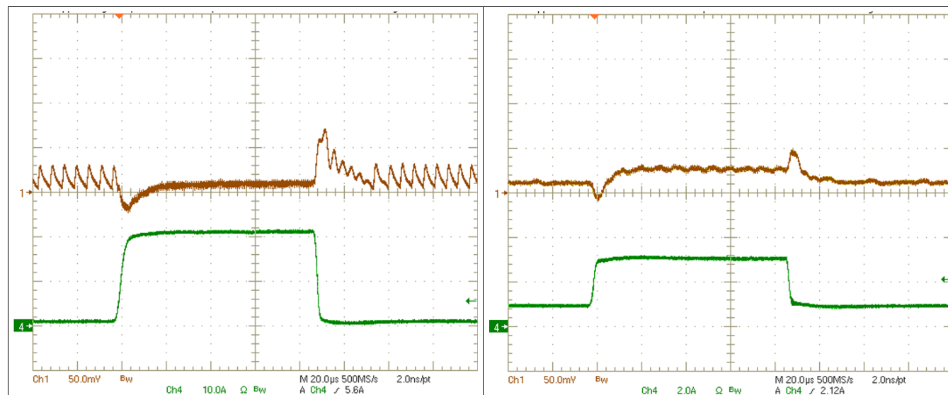
Figure 7-4. BUCK2 Controller Load Transient
