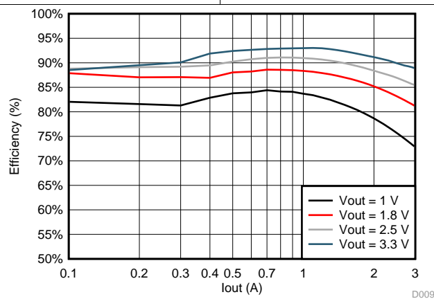
图 4-5. Converter Efficiency at V_{IN} = 5\text{ V}
