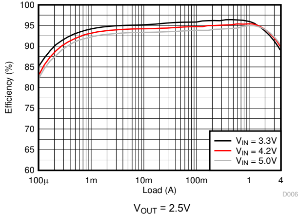
图 8-15. Efficiency
