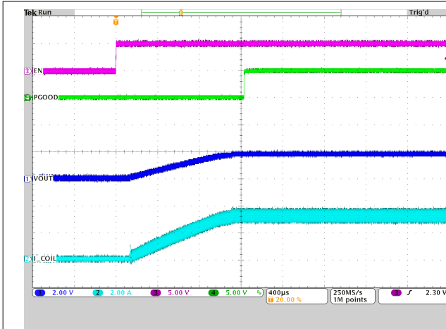
Load = 0.6 \Omega TPS62826A/7A
