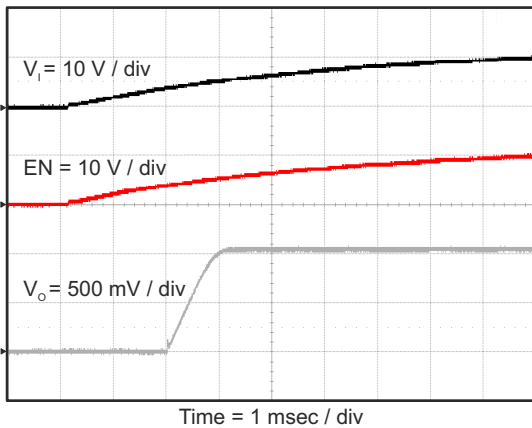
图 8-27. Tps563200 Start-up Relative to V i
