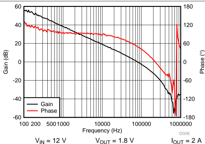
图 40. Loop Response
