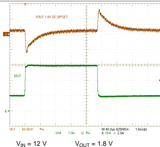
图 41. Transient Response
