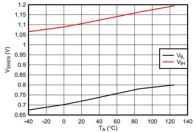
图 7-14. SWEN Pin Logic Thresholds Across Temperature
