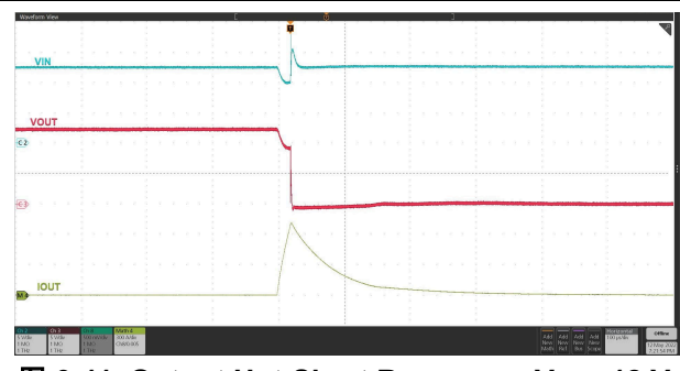
图 9-11. Output Hot-Short Response: V_{IN} = 12 V, R_{IMON} = 200 \Omega , R_{REF} = 40.2 k \Omega , and OUT Shorted to GND
