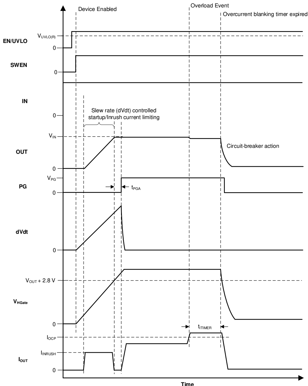
图 8-8. TPS25984x PG Timing Diagram
