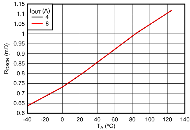
图 7-1. ON Resistance Across Temperature
