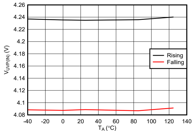
图 7-3. VIN Undervoltage Thresholds Across Temperature
