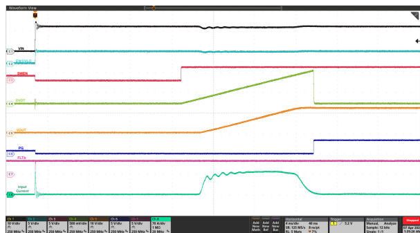
图 9-6. Input Hot Plug: V_{IN} Stepped Up from 0 V to 12 V, C_{LOAD} = 50 mF, C_{DVT} = 33 nF, and R_{ILIM} on Each Device = 442 \Omega
