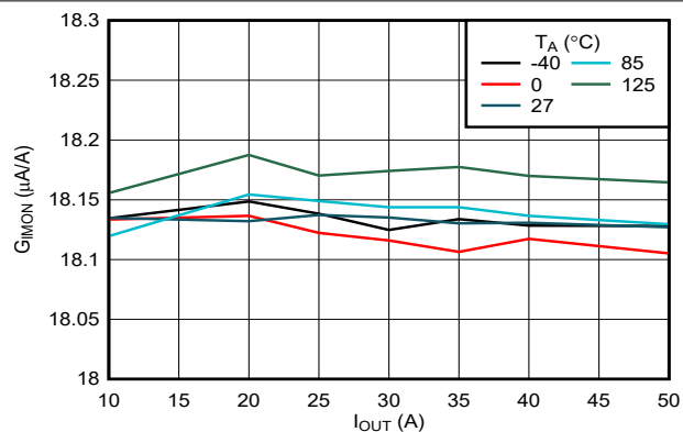
图 7-8. IMON Gain Across Load and Temperature
