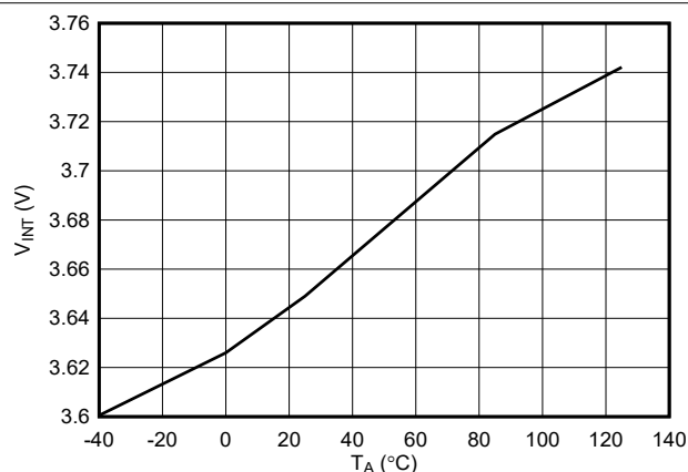
图 7-11. ITIMER Pin Internal Pullup Voltage Across Temperature
