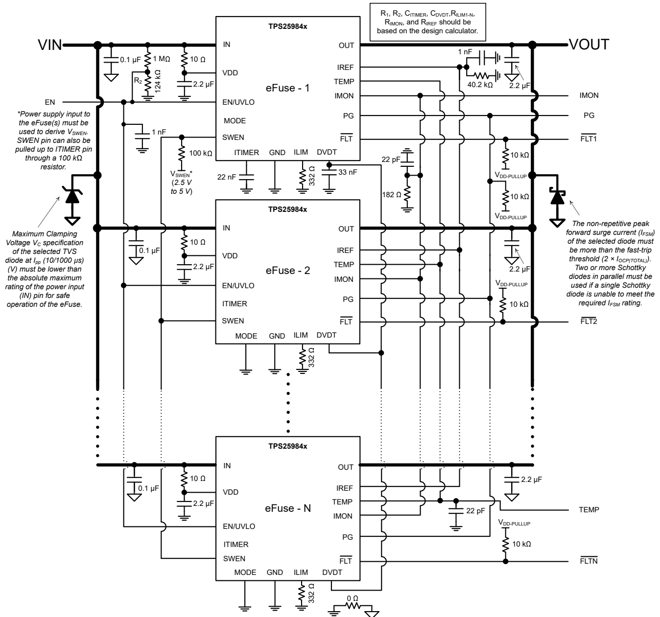
图 9-5. Application Schematic for a 12-V, 3.3-kW Power Path Protection Circuit
