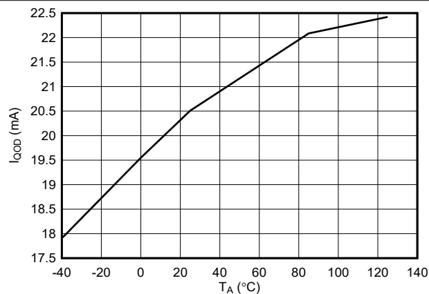
图 7-17. QOD Sink Current Across Temperature
