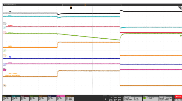
图 9-10. Circuit-Breaker Response: V_{IN} = 12 V, C_{TIMER} = 22 nF, C_{LOAD} = 50 mF, R_{IMON} = 200 \Omega , R_{REF} = 40.2 k \Omega , and Load Current Stepped up From 250 A to 400 A for > 20 ms
