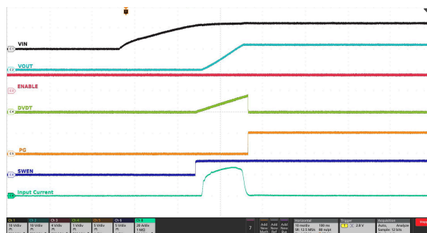
图 7-20. Power Up Control Using Input Supply
