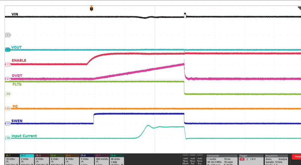
图 7-32. Overcurrent Protection Response (Circuit-Breaker)
