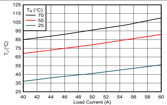
图 7-18. Junction Temperature vs Load Current (No Air-Flow)
