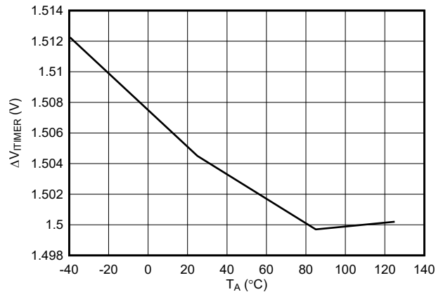
图 7-13. ITIMER Pin Discharge Differential Voltage Threshold Across Temperature
