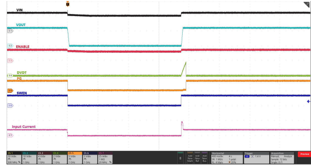
图 7-26. Power Up and Down Sequencing Using SWEN Pin
