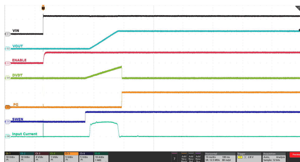
图 7-19. Input Hot-plug With Insertion Delay
