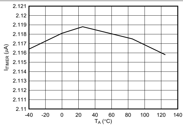
图 7-12. ITIMER Pin Discharge Current Across Temperature
