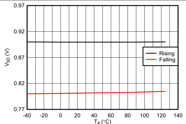
图 7-6. EN/UVLO Based Thresholds for Device Shutdown Across Temperature
