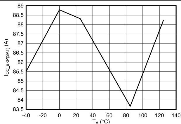
图 7-9. Backup Overcurrent Protection Threshold (Start-up) Accuracy
