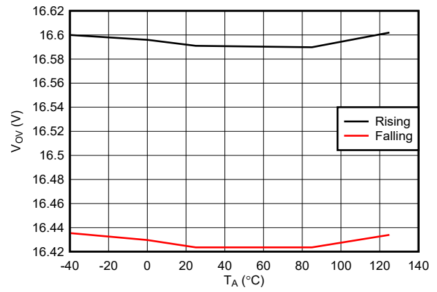
图 7-4. VIN Overvoltage Protection Thresholds Across Temperature
