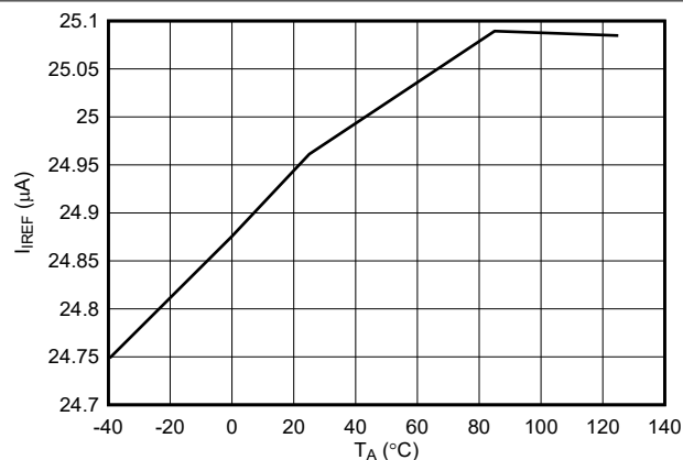
图 7-7. IREF Charging Current Across Temperature
