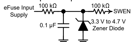
图 9-14. Zener Regulator Used as Pullup Supply for SWEN
