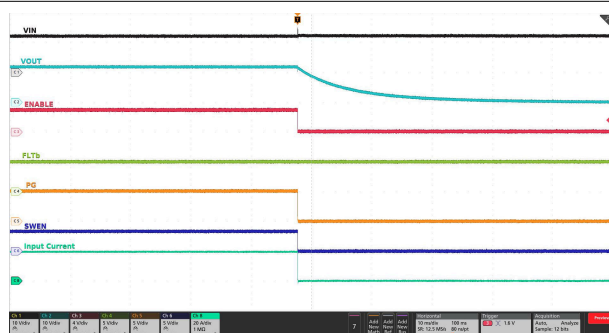
图 7-21. Power Up and Down Sequencing Using EN/UVLO Pin
