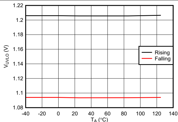
图 7-5. EN/UVLO Thresholds For FET Turn-off Across Temperature
