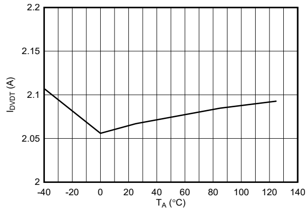
图 7-15. DVDVT Charging Current Across Temperature
