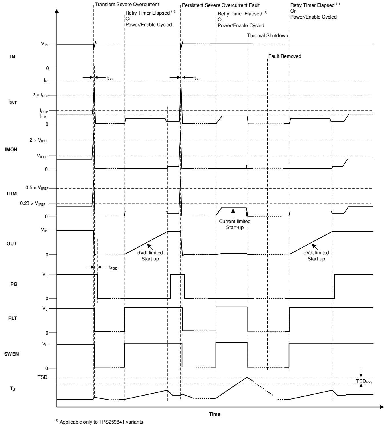
图 8-5. Short-Circuit Response
