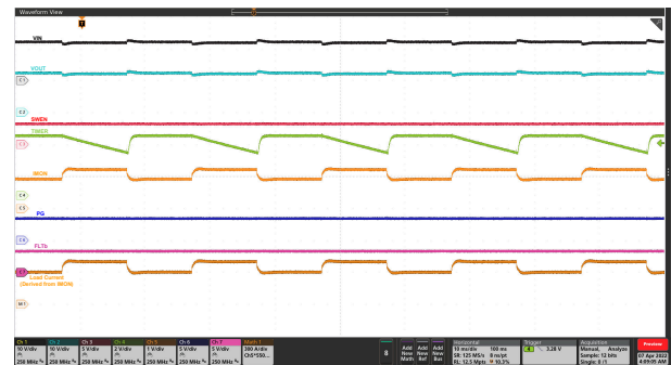
图 9-9. Transient Overload: V_{IN} = 12 V, C_{TIMER} = 22 nF, C_{LOAD} = 50 mF, R_{IMON} = 200 \Omega , R_{REF} = 40.2 k \Omega , and Load Current Stepped from 250 A to 300 A then 250 A within 10 ms
