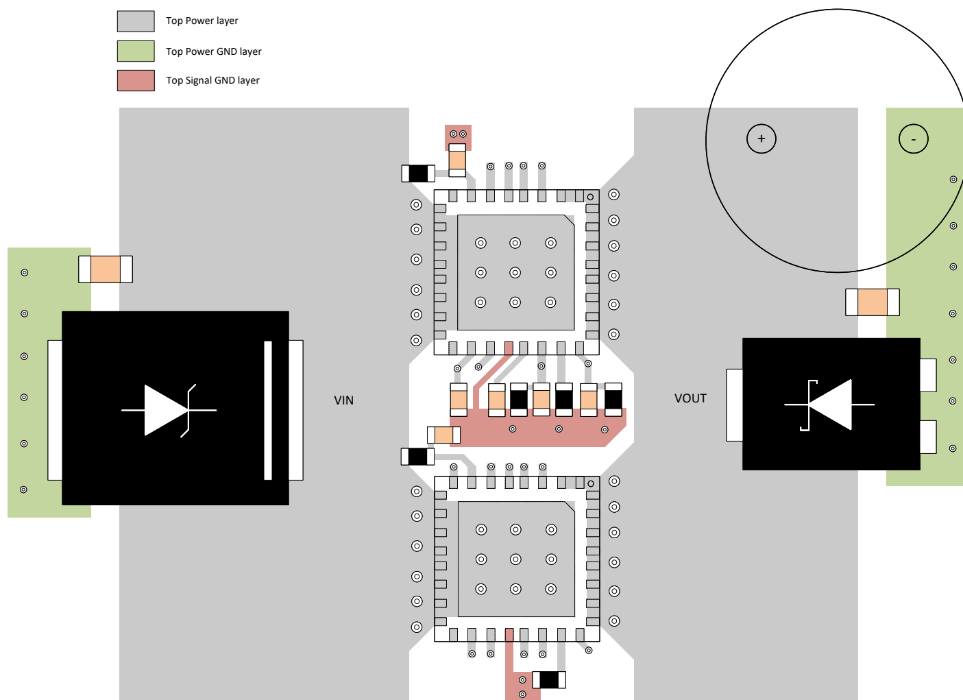
图 9-17. TPS25984x Two Parallel Devices Layout Example
