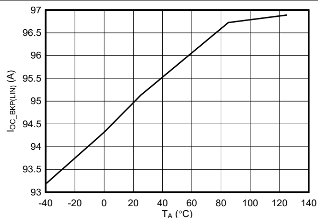
图 7-10. Backup Overcurrent Protection Threshold (Steady-State) Accuracy
