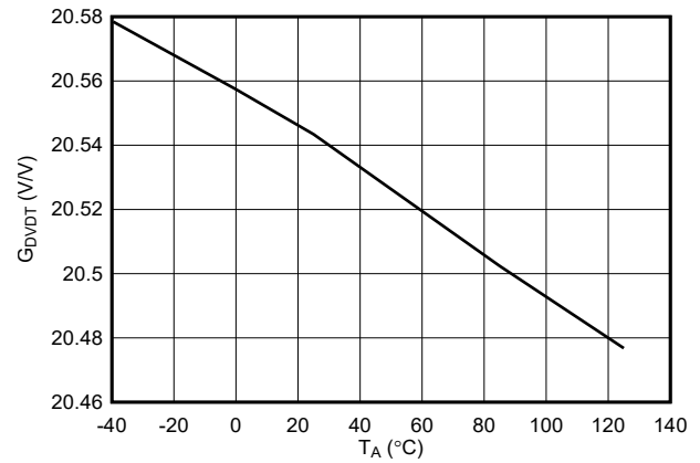
图 7-16. DVDVT Gain Across Temperature
