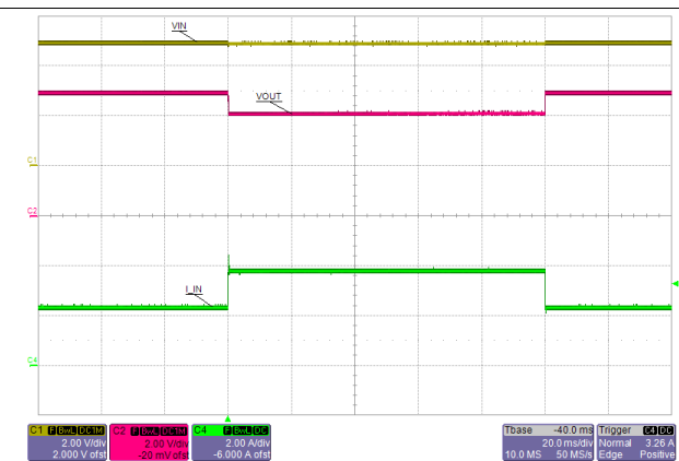
Figure 38. Transient: Overload Current Limit
