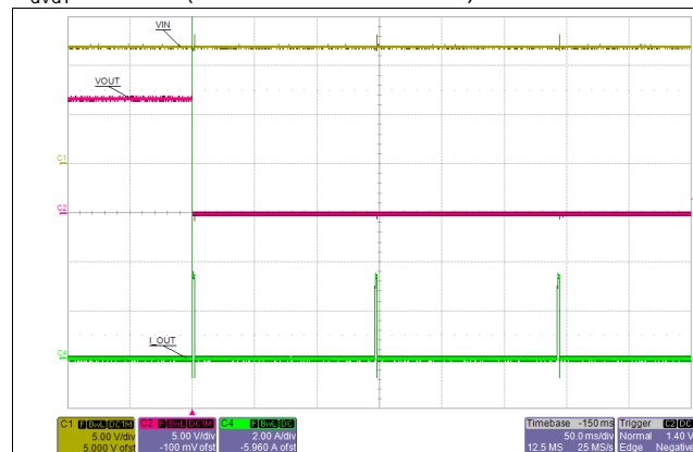
Figure 37. Transient: Thermal Fault Auto-Retry
