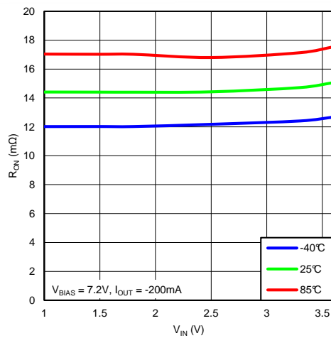
Figure 7. R_{ON} vs. V_{IN} ( V_{BIAS} = 7.2V )
