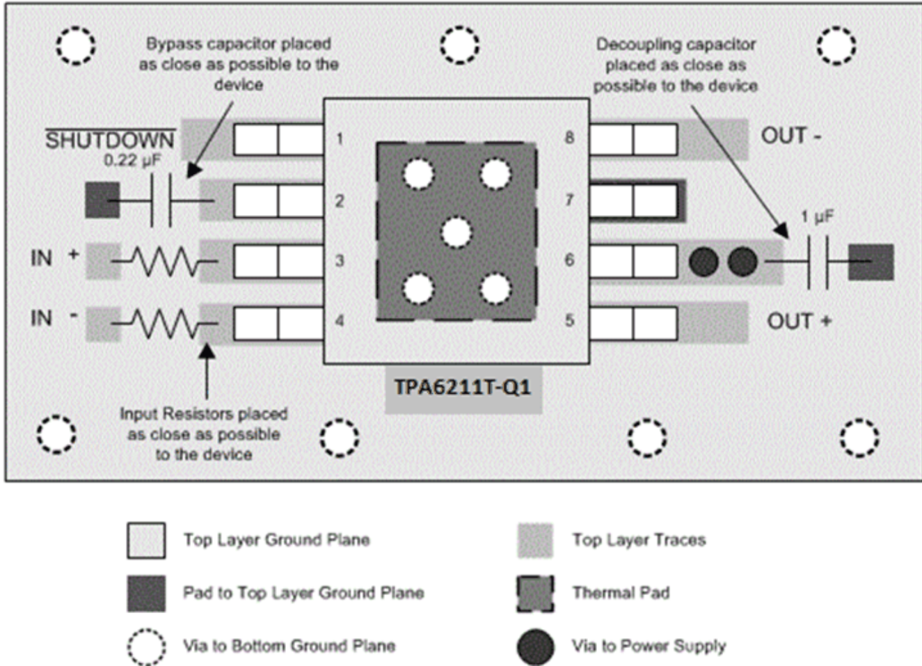
图 9-1. TPA6211T-Q1 8-Pin HVSSOP (DGN) Board Layout
