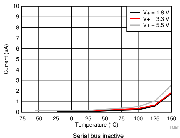
图 6-6. Quiescent Current in Shutdown Mode
