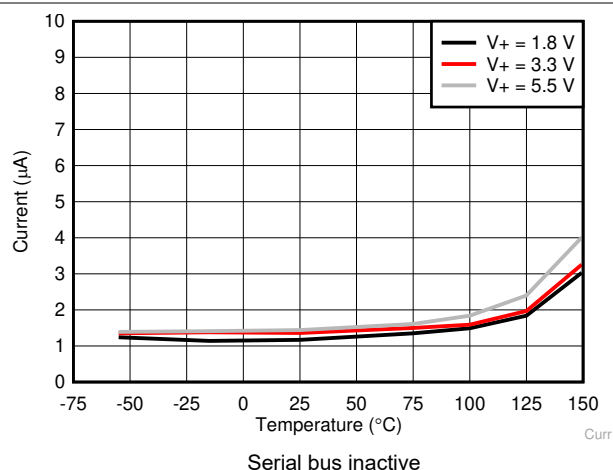
图 6-7. Quiescent Current in Standby Mode
