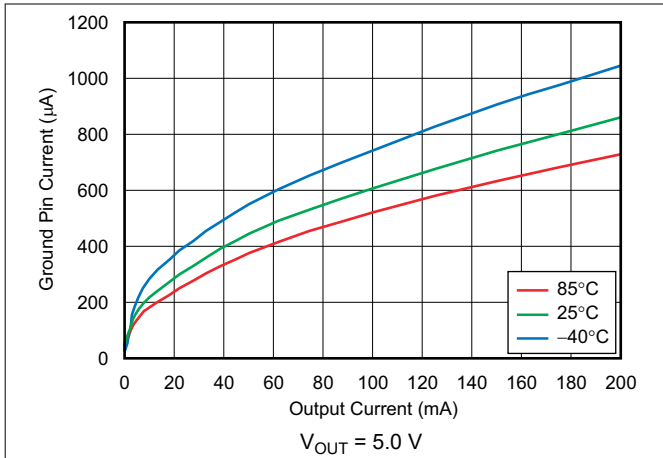
图 6-25. Ground Pin Current vs Output Current
