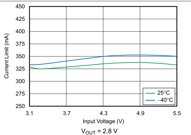
图 6-30. Current Limit vs Input Voltage
