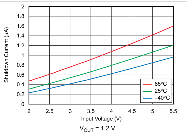
图 6-26. Shutdown Current vs Input Voltage
