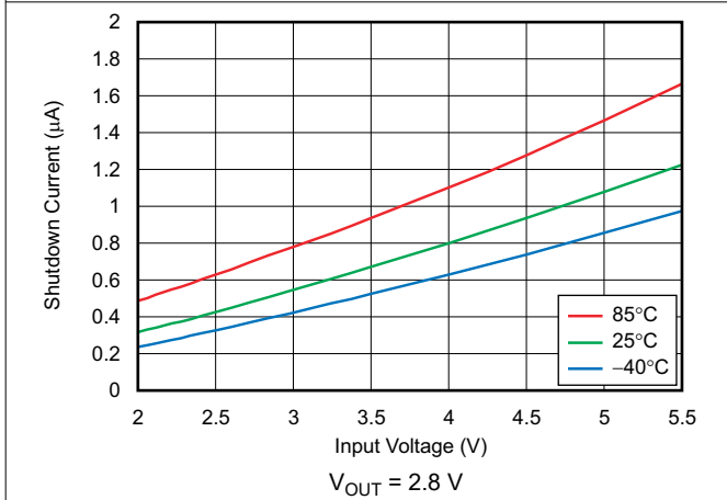
图 6-27. Shutdown Current vs Input Voltage
