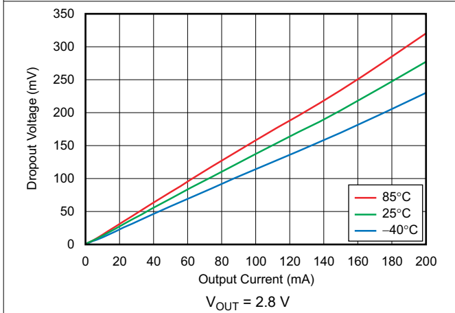
图 6-15. Dropout Voltage vs Output Current
