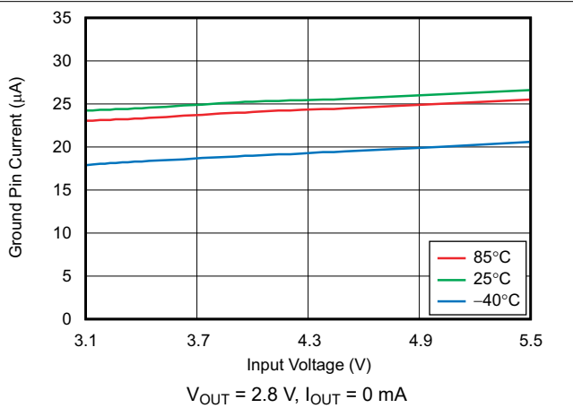
图 6-18. Ground Pin Current vs Input Voltage
