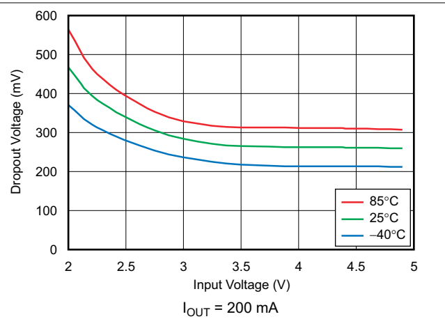
图 6-14. Dropout Voltage vs Input Voltage
