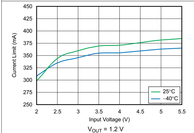
图 6-29. Current Limit vs Input Voltage
