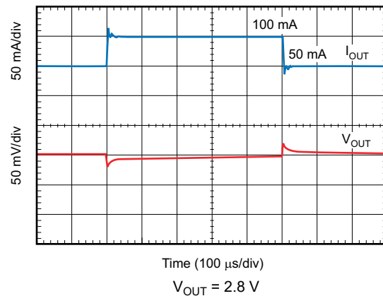
图 6-42. Load Transient Response
