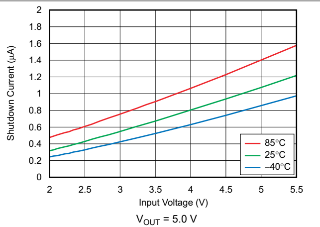
图 6-28. Shutdown Current vs Input Voltage
