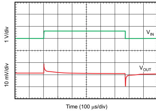
图 6-50. Line Transient Response
