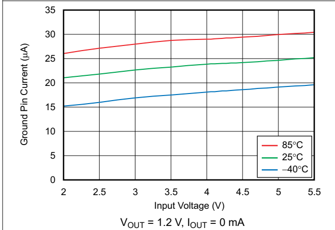
图 6-17. Ground Pin Current vs Input Voltage
