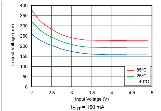
图 6-13. Dropout Voltage vs Input Voltage
