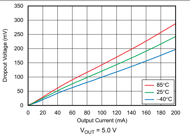
图 6-16. Dropout Voltage vs Output Current
