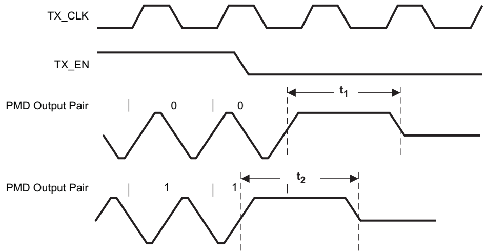
Figure 9-14. 10Base-T Transmit Timing (End of Packet)
