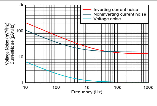
图 7-16. Noise vs Frequency
