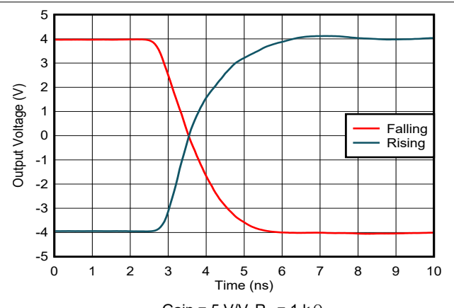
图 7-18. Settling Time
