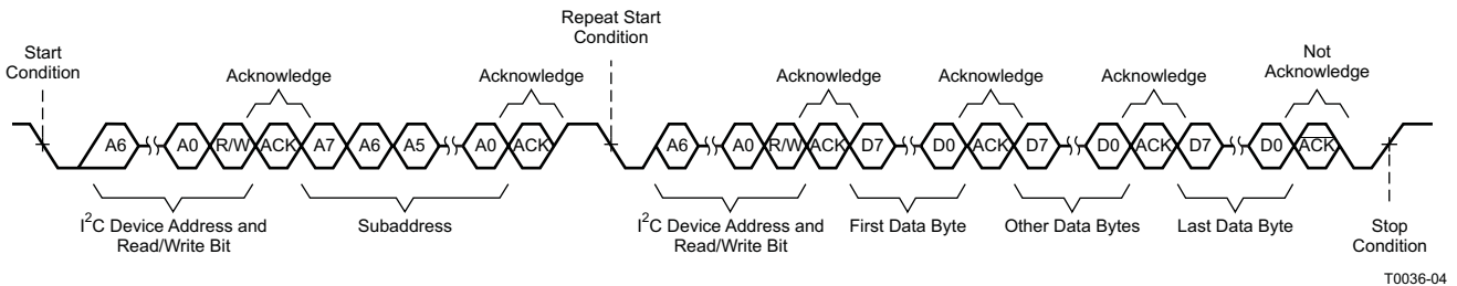
图 32. Multi-Byte Read Transfer Timing
