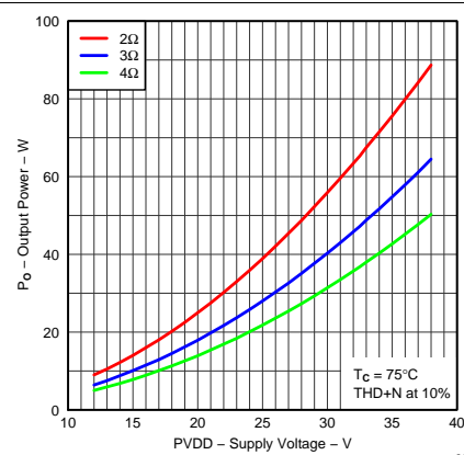
图 10. Output Power vs Supply Voltage
