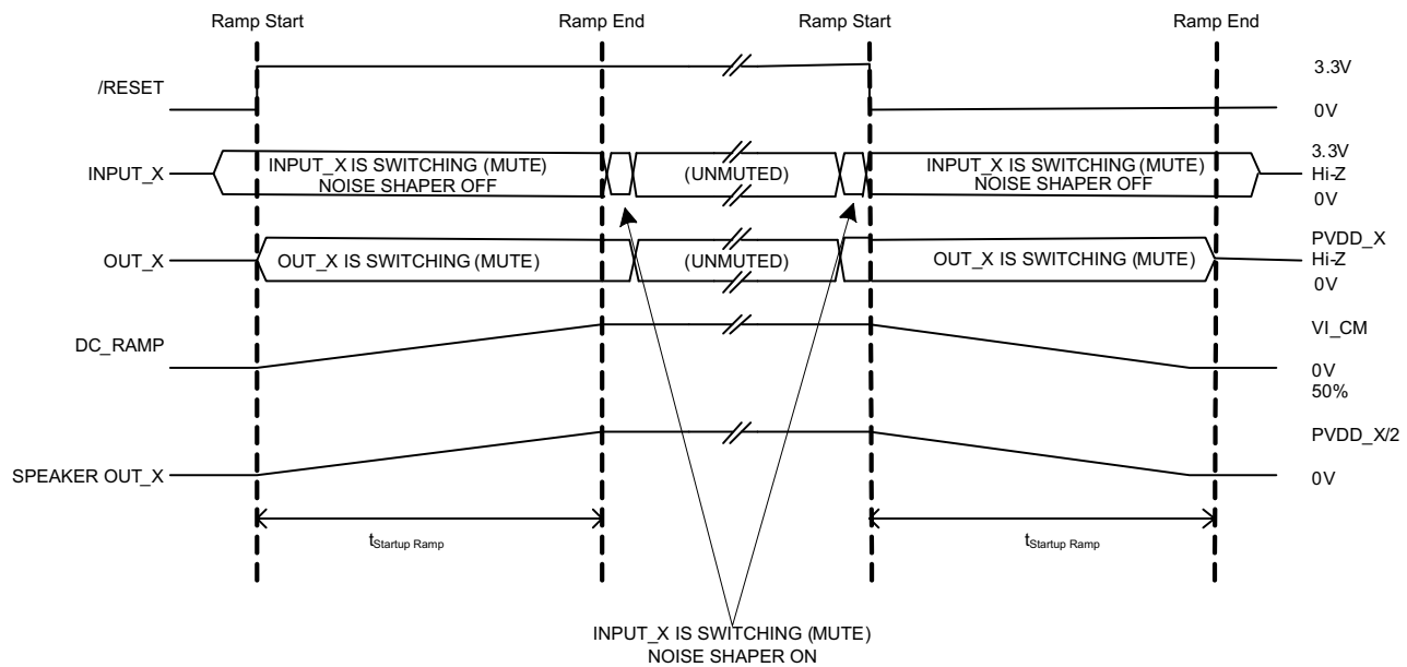
图 15. Start-up/Shutdown Ramp
