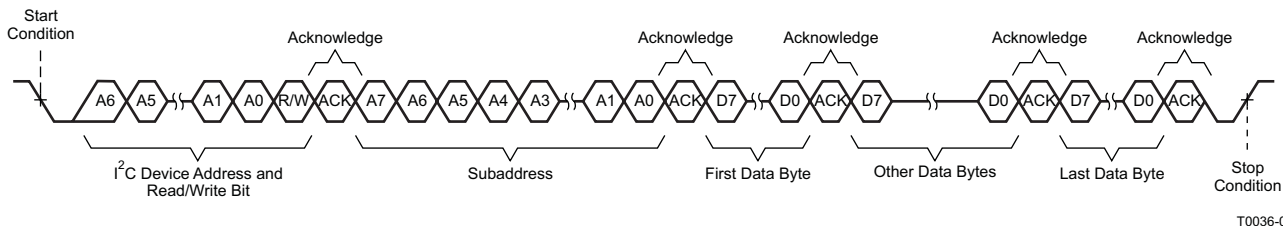
Figure 15. Sequential Write Transfer
