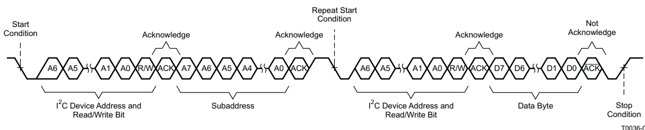
Figure 16. Random Read Transfer
