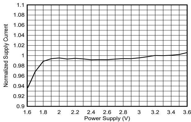
图 7-5. Active Current vs Power Supply
