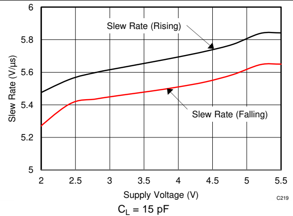
图 34. Slew Rate vs Supply Voltage
