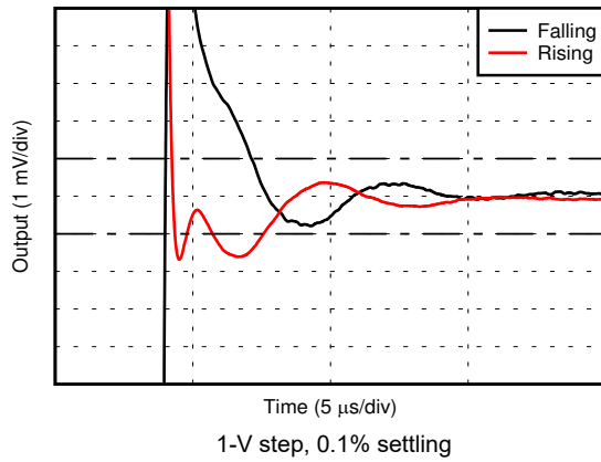
图 6-35. Settling Time
