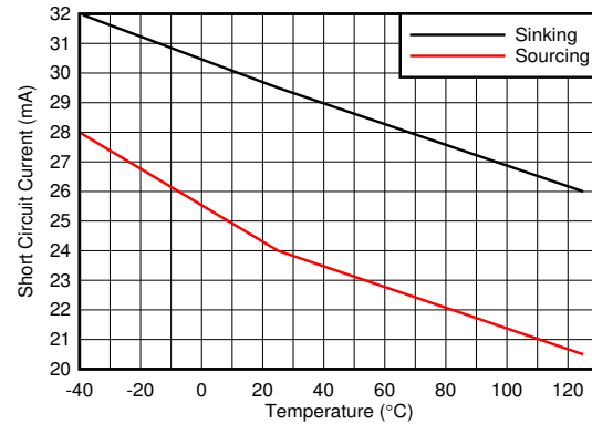
图 6-36. Short Circuit Current vs Temperature
