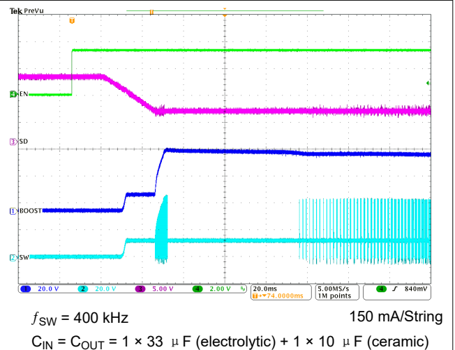
图 8-4. Typical Start-Up
