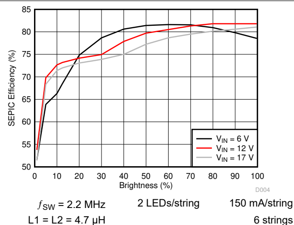
图 6-5. SEPIC Efficiency
