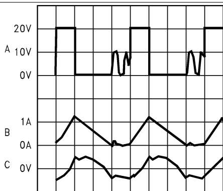
1 \mu\text{sec}/\text{Div} Discontinuous Mode Switching Waveforms V_{\text{IN}} = 20\text{ V} , V_{\text{OUT}} = 5\text{ V} , I_{\text{LOAD}} = 500\text{ mA} L = 10\ \mu\text{H} , C_{\text{OUT}} = 400\ \mu\text{F} , C_{\text{OUTESR}} = 13\ \text{m}\Omega A: V_{\text{SW}} Pin Voltage, 10 V/div B: Inductor Current, 1 A/div C: Output Ripple Voltage, 20 mV/div AC-Coupled
