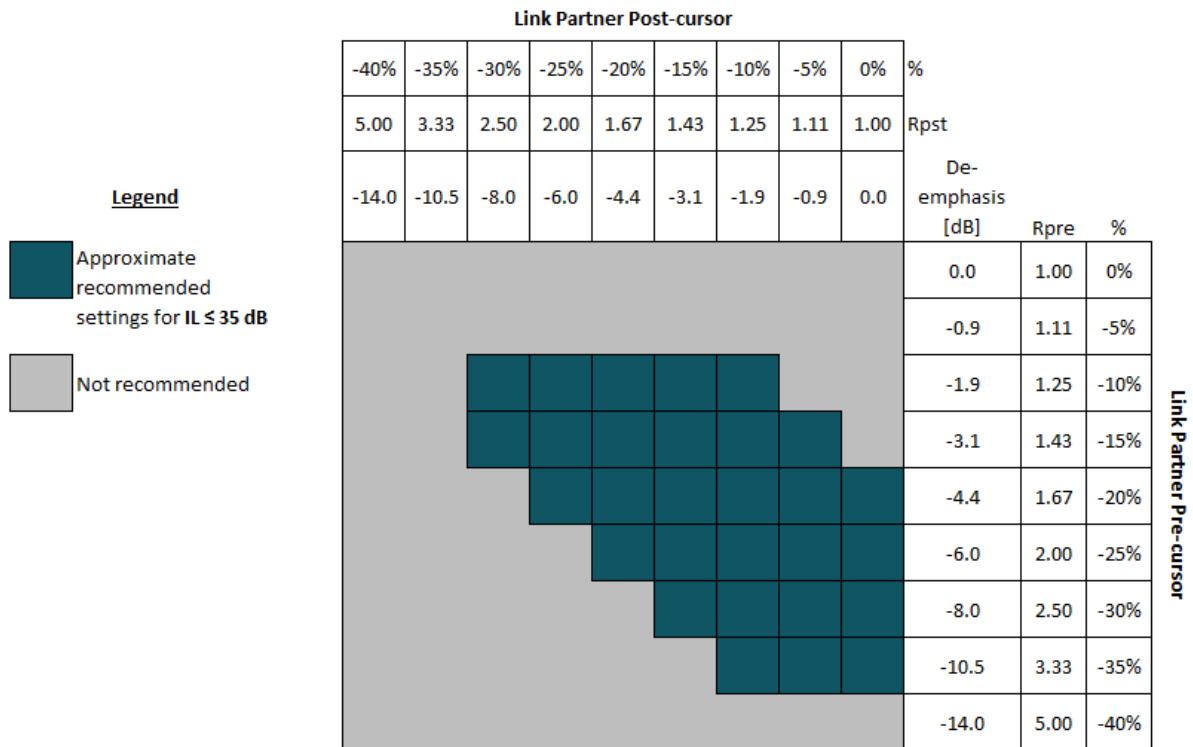
图 6-9. Guideline for Link partner FIR Settings When IL ≤ 35dB
