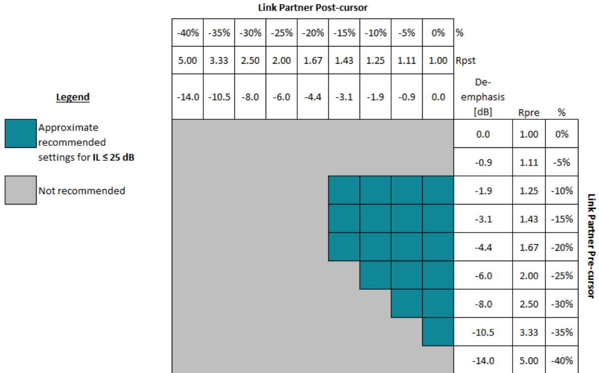
图 6-8. Guideline for Link partner FIR Settings When IL ≤ 25dB
