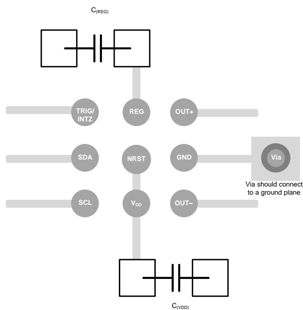
图 98. Layout without NRST Functionality
