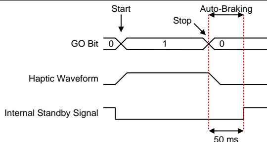
图 36. Playback Start and stop Trigger (Internal GO bit) (RTP or Waveform Sequencer)
